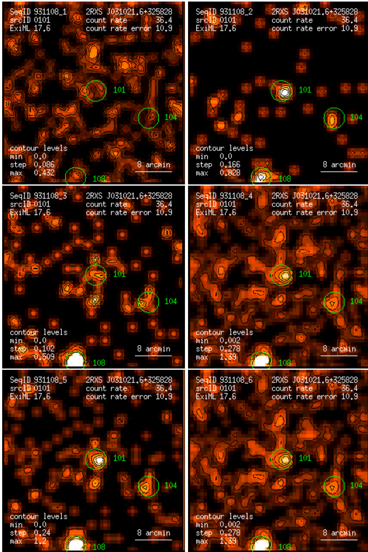
Figure 101: RASS 931108: detection 0101: band rate images, Gaussian filter: (1) PSPC channels 11 – 41, (2) 52 – 90, (3) 91 – 201, (4) 11 – 235, (5) 52 – 201, (6) 11 – 201. Broad band rates in counts/ks. Band rate contour levels in counts/ks/arcmin 2 .
