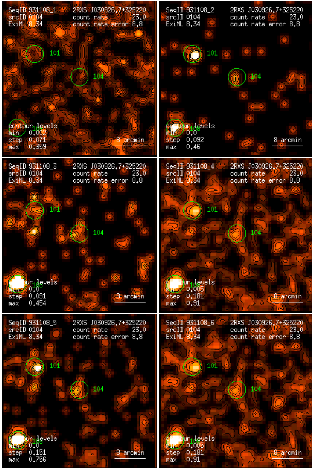
Figure 104: RASS 931108: detection 0104: band rate images, Gaussian filter: (1) PSPC channels 11 – 41, (2) 52 – 90, (3) 91 – 201, (4) 11 – 235, (5) 52 – 201, (6) 11 – 201. Broad band rates in counts/ks. Band rate contour levels in counts/ks/arcmin 2 .
