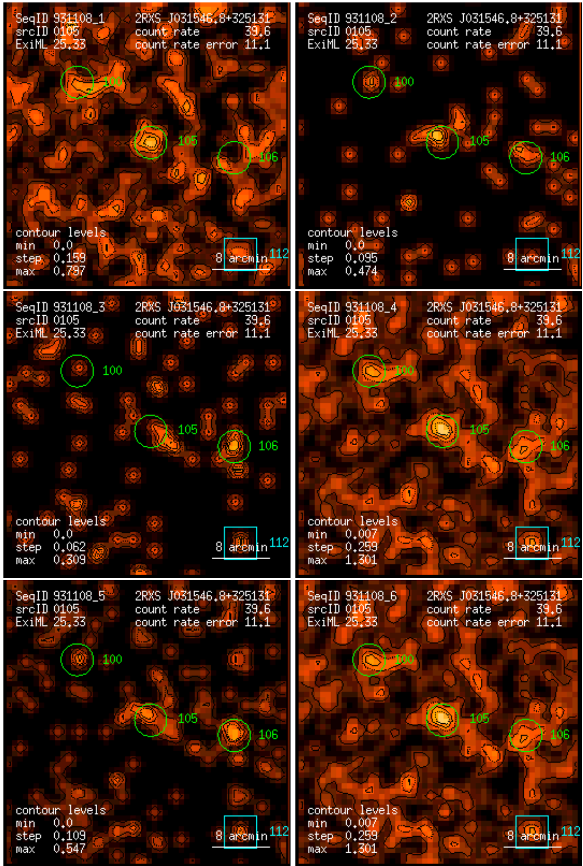
Figure 105: RASS 931108: detection 0105: band rate images, Gaussian filter: (1) PSPC channels 11 – 41, (2) 52 – 90, (3) 91 – 201, (4) 11 – 235, (5) 52 – 201, (6) 11 – 201. Broad band rates in counts/ks. Band rate contour levels in counts/ks/arcmin 2 .
