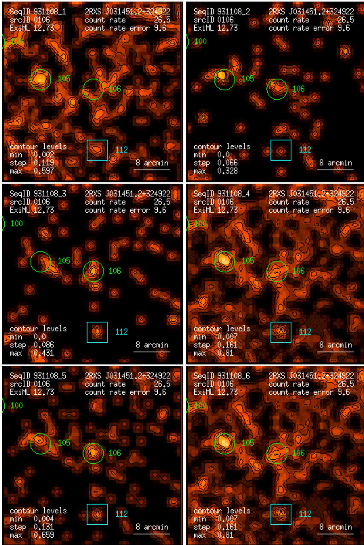
Figure 106: RASS 931108: detection 0106: band rate images, Gaussian filter: (1) PSPC channels 11 – 41, (2) 52 – 90, (3) 91 – 201, (4) 11 – 235, (5) 52 – 201, (6) 11 – 201. Broad band rates in counts/ks. Band rate contour levels in counts/ks/arcmin 2 .
