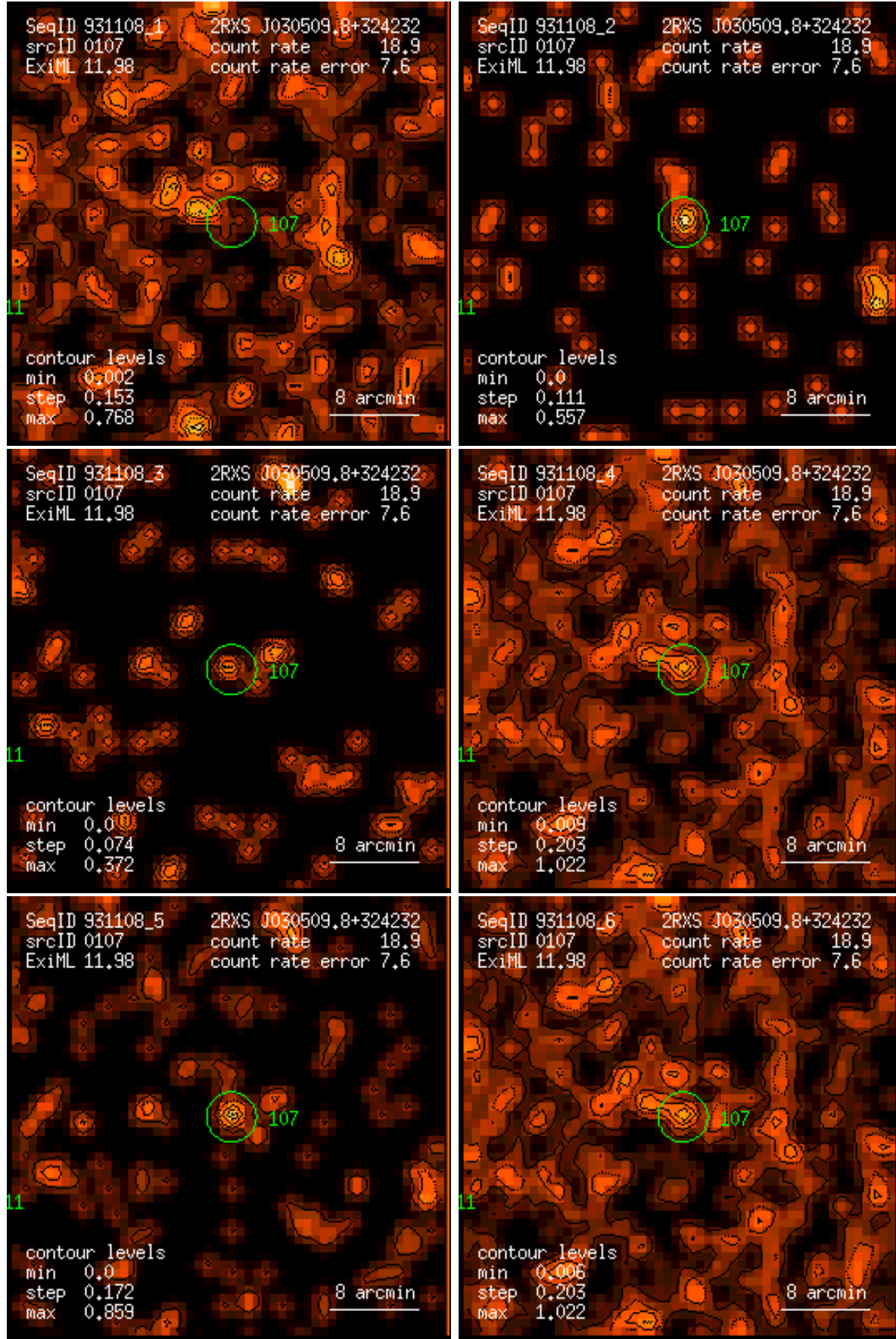
Figure 107: RASS 931108: detection 0107: band rate images, Gaussian filter: (1) PSPC channels 11 – 41, (2) 52 – 90, (3) 91 – 201, (4) 11 – 235, (5) 52 – 201, (6) 11 – 201. Broad band rates in counts/ks. Band rate contour levels in counts/ks/arcmin 2 .
