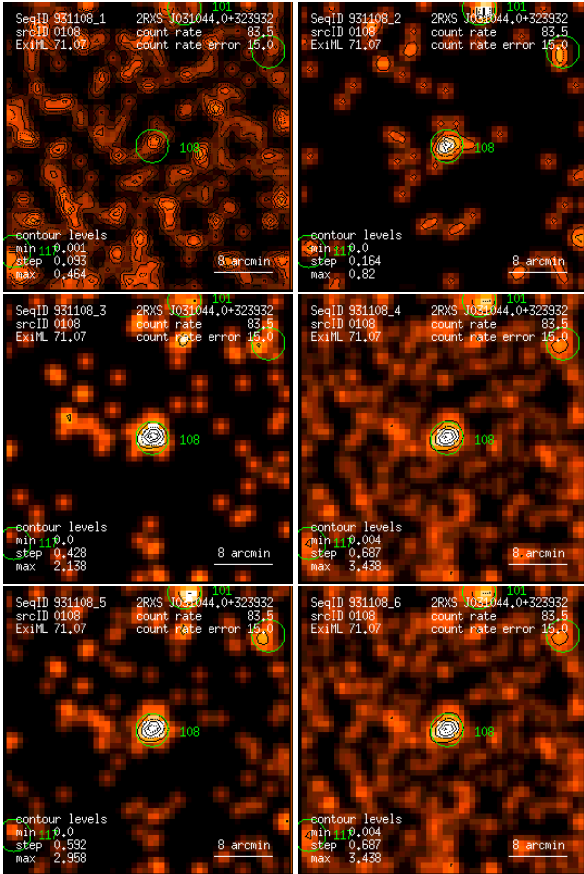
Figure 108: RASS 931108: detection 0108: band rate images, Gaussian filter: (1) PSPC channels 11 – 41, (2) 52 – 90, (3) 91 – 201, (4) 11 – 235, (5) 52 – 201, (6) 11 – 201. Broad band rates in counts/ks. Band rate contour levels in counts/ks/arcmin 2 .
