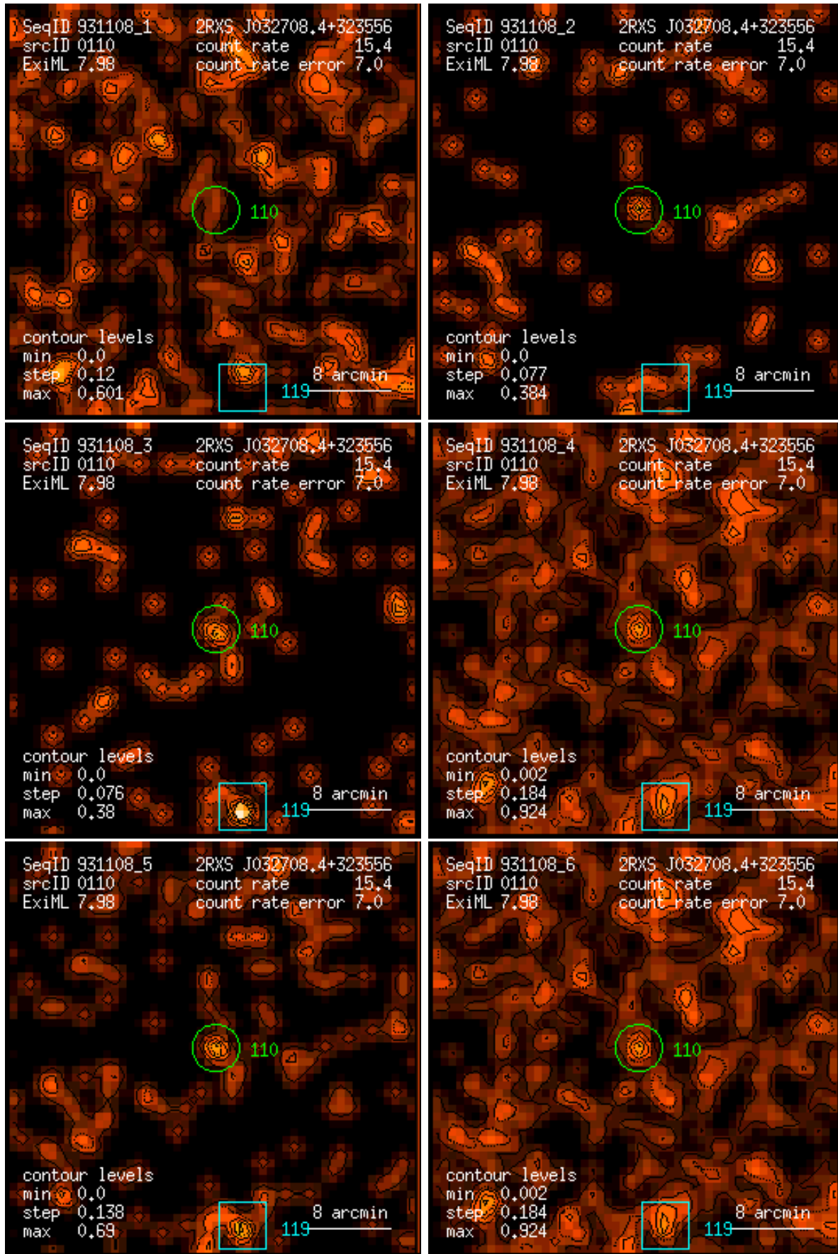
Figure 110: RASS 931108: detection 0110: band rate images, Gaussian filter: (1) PSPC channels 11 – 41, (2) 52 – 90, (3) 91 – 201, (4) 11 – 235, (5) 52 – 201, (6) 11 – 201. Broad band rates in counts/ks. Band rate contour levels in counts/ks/arcmin 2 .
