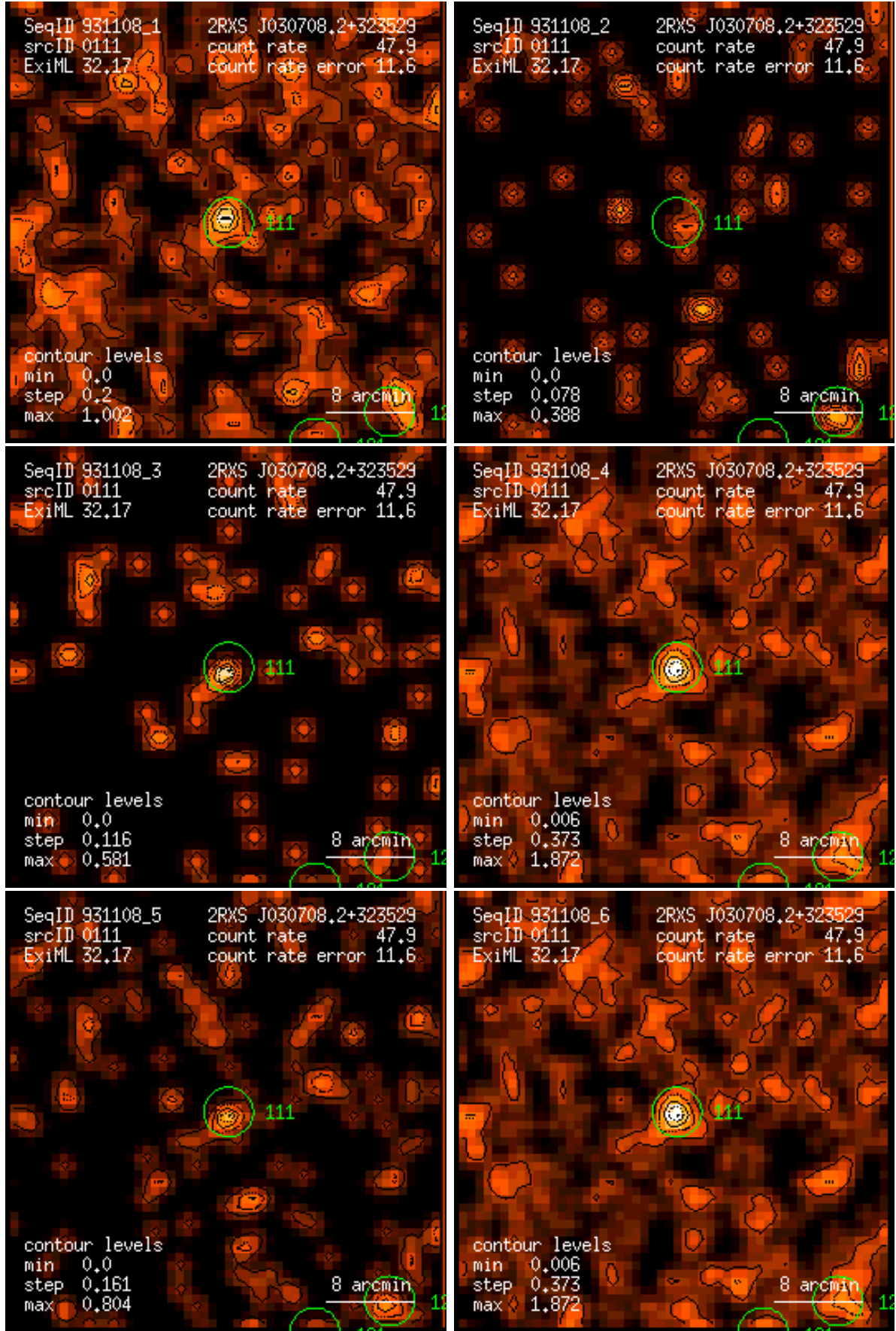
Figure 111: RASS 931108: detection 0111: band rate images, Gaussian filter: (1) PSPC channels 11 – 41, (2) 52 – 90, (3) 91 – 201, (4) 11 – 235, (5) 52 – 201, (6) 11 – 201. Broad band rates in counts/ks. Band rate contour levels in counts/ks/arcmin 2 .
