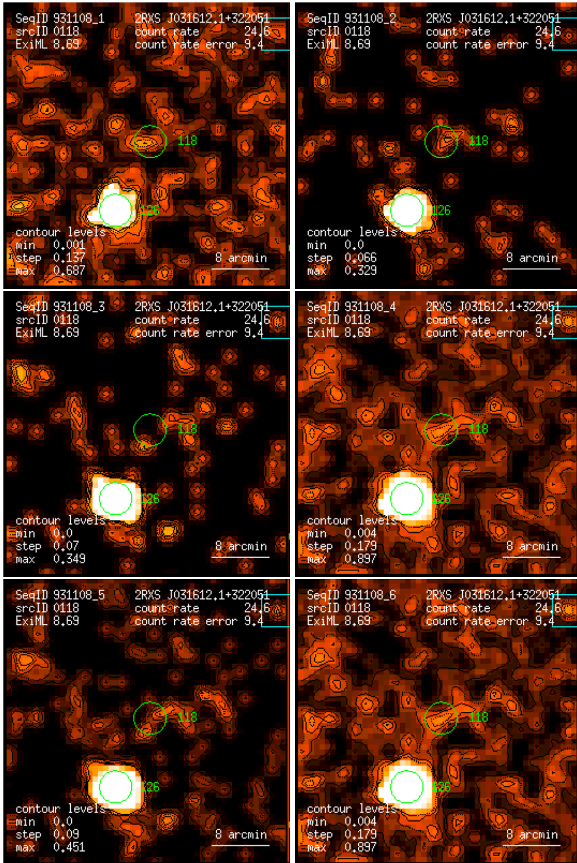
Figure 118: RASS 931108: detection 0118: band rate images, Gaussian filter: (1) PSPC channels 11 – 41, (2) 52 – 90, (3) 91 – 201, (4) 11 – 235, (5) 52 – 201, (6) 11 – 201. Broad band rates in counts/ks. Band rate contour levels in counts/ks/arcmin 2 .
