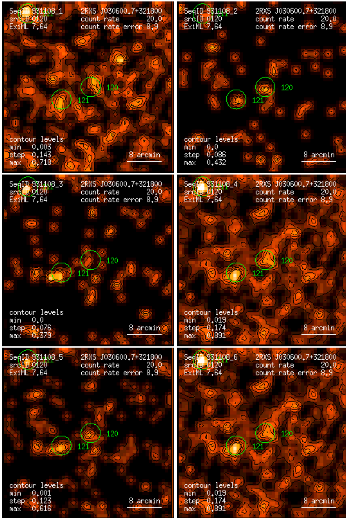
Figure 120: RASS 931108: detection 0120: band rate images, Gaussian filter: (1) PSPC channels 11 – 41, (2) 52 – 90, (3) 91 – 201, (4) 11 – 235, (5) 52 – 201, (6) 11 – 201. Broad band rates in counts/ks. Band rate contour levels in counts/ks/arcmin 2 .
