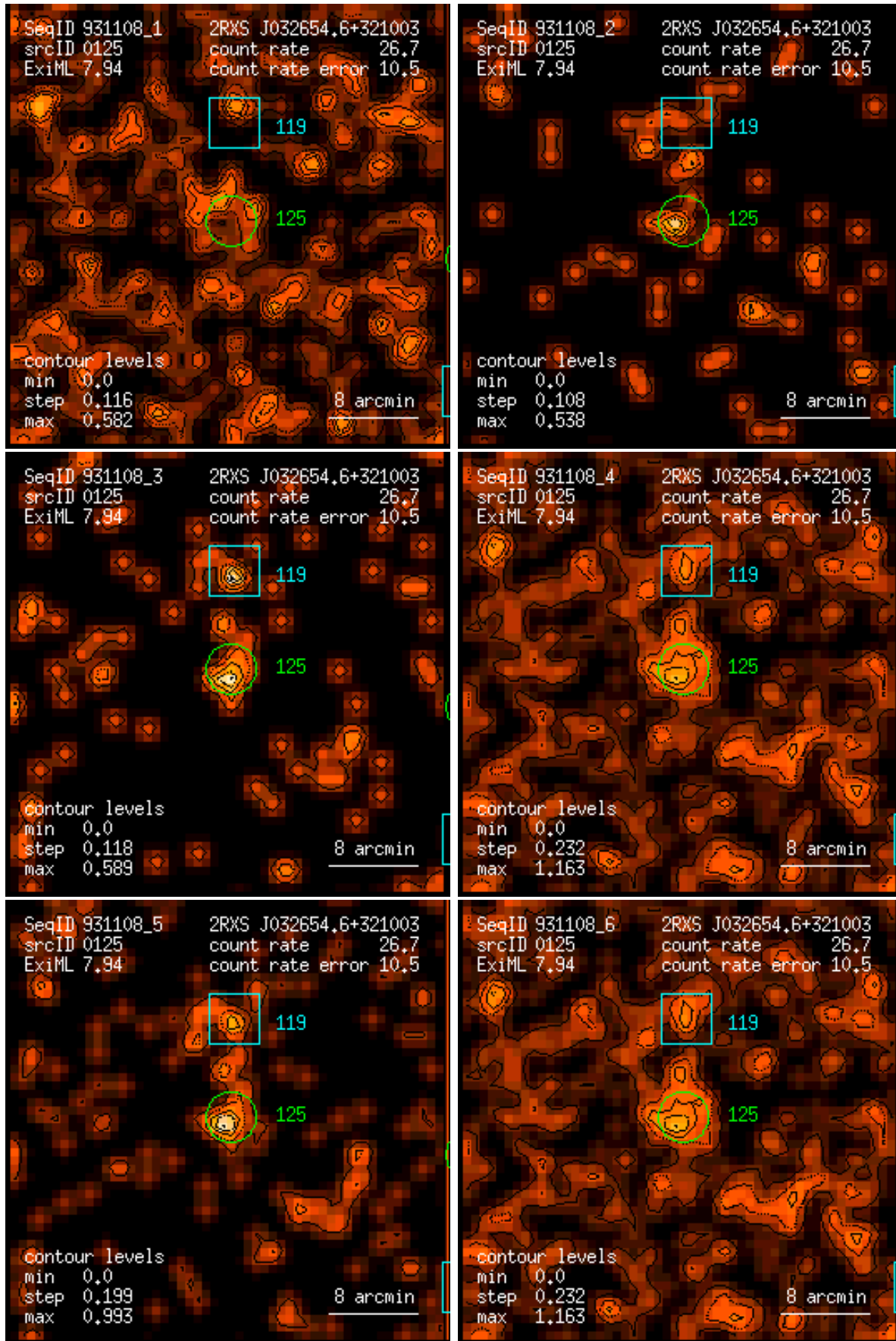
Figure 125: RASS 931108: detection 0125: band rate images, Gaussian filter: (1) PSPC channels 11 – 41, (2) 52 – 90, (3) 91 – 201, (4) 11 – 235, (5) 52 – 201, (6) 11 – 201. Broad band rates in counts/ks. Band rate contour levels in counts/ks/arcmin 2 .
