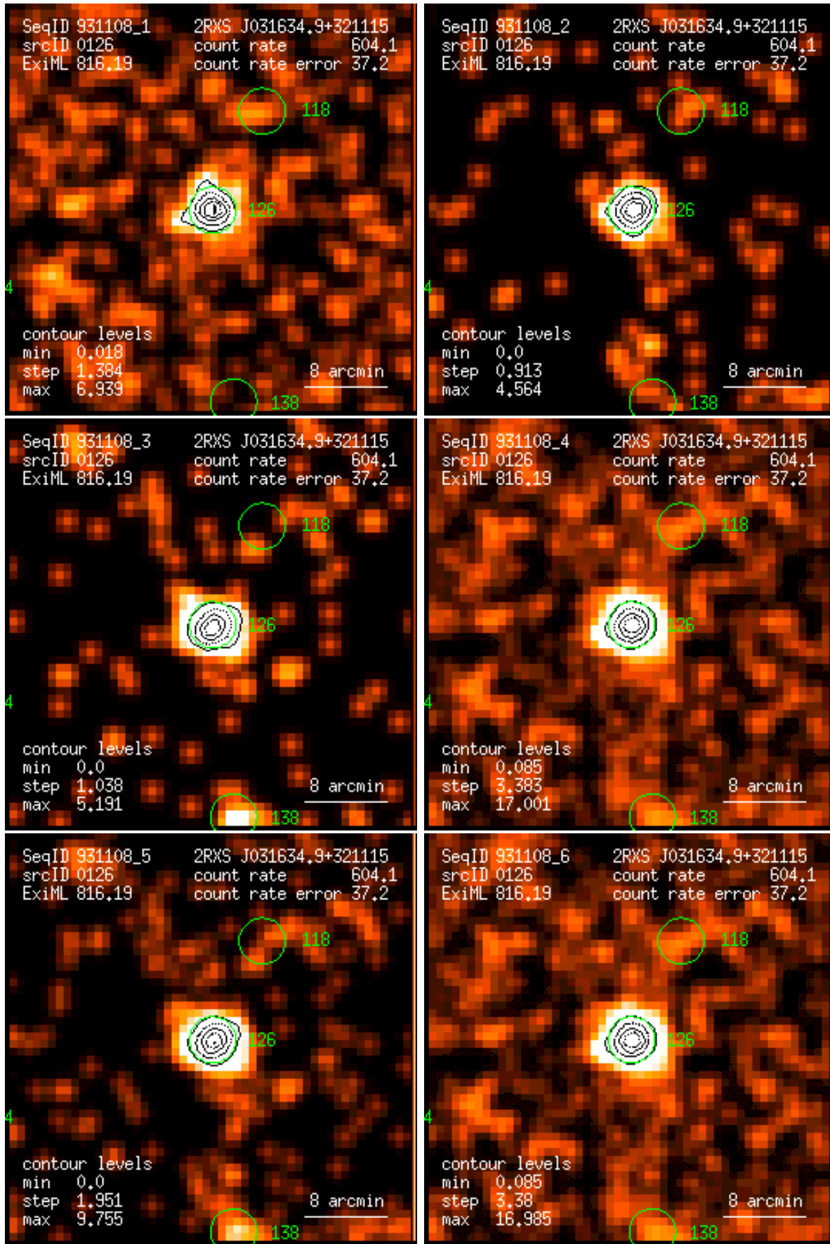
Figure 126: RASS 931108: detection 0126: band rate images, Gaussian filter: (1) PSPC channels 11 – 41, (2) 52 – 90, (3) 91 – 201, (4) 11 – 235, (5) 52 – 201, (6) 11 – 201. Broad band rates in counts/ks. Band rate contour levels in counts/ks/arcmin 2 .
