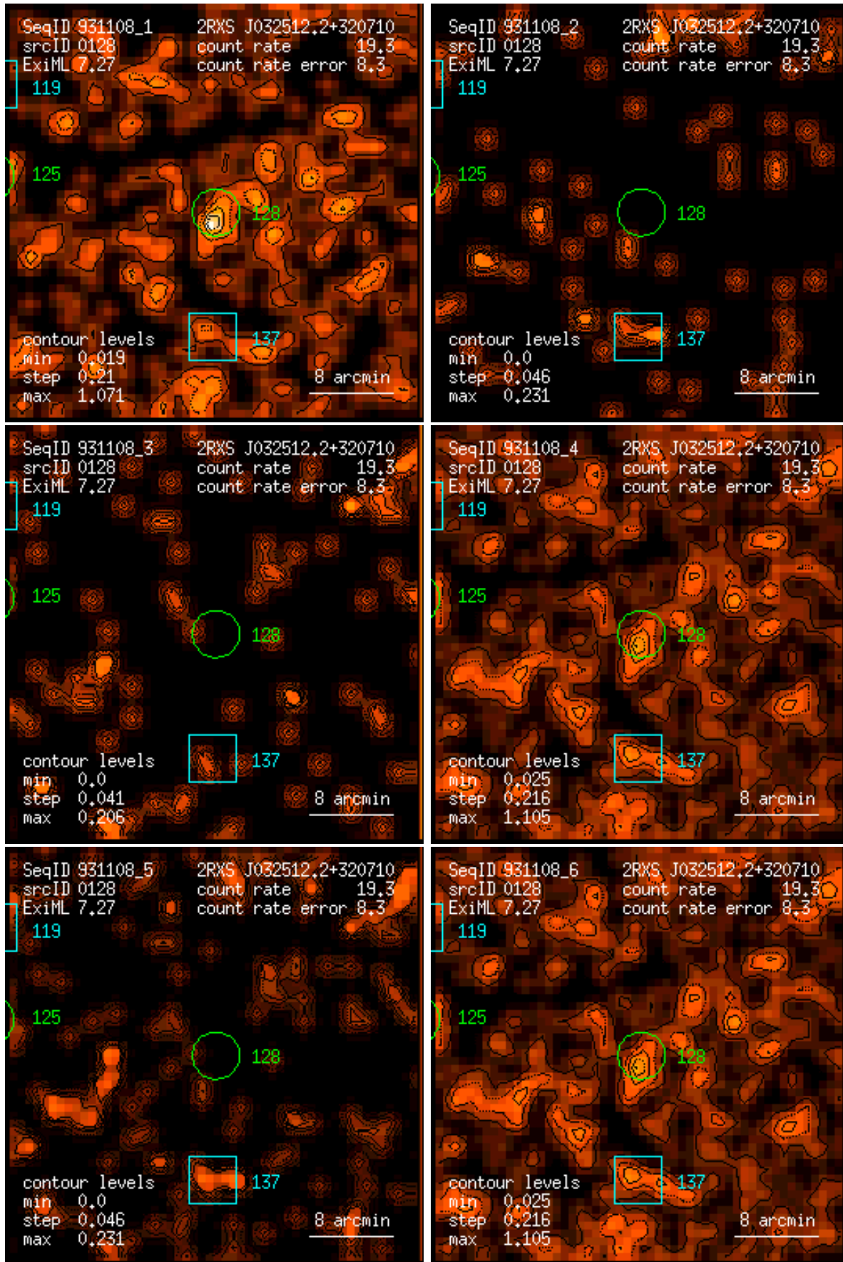
Figure 128: RASS 931108: detection 0128: band rate images, Gaussian filter: (1) PSPC channels 11 – 41, (2) 52 – 90, (3) 91 – 201, (4) 11 – 235, (5) 52 – 201, (6) 11 – 201. Broad band rates in counts/ks. Band rate contour levels in counts/ks/arcmin 2 .
