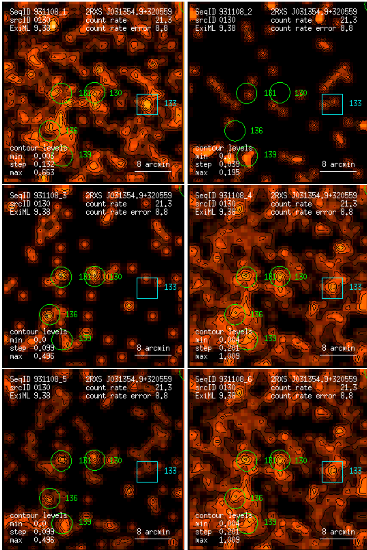
Figure 130: RASS 931108: detection 0130: band rate images, Gaussian filter: (1) PSPC channels 11 – 41, (2) 52 – 90, (3) 91 – 201, (4) 11 – 235, (5) 52 – 201, (6) 11 – 201. Broad band rates in counts/ks. Band rate contour levels in counts/ks/arcmin 2 .
