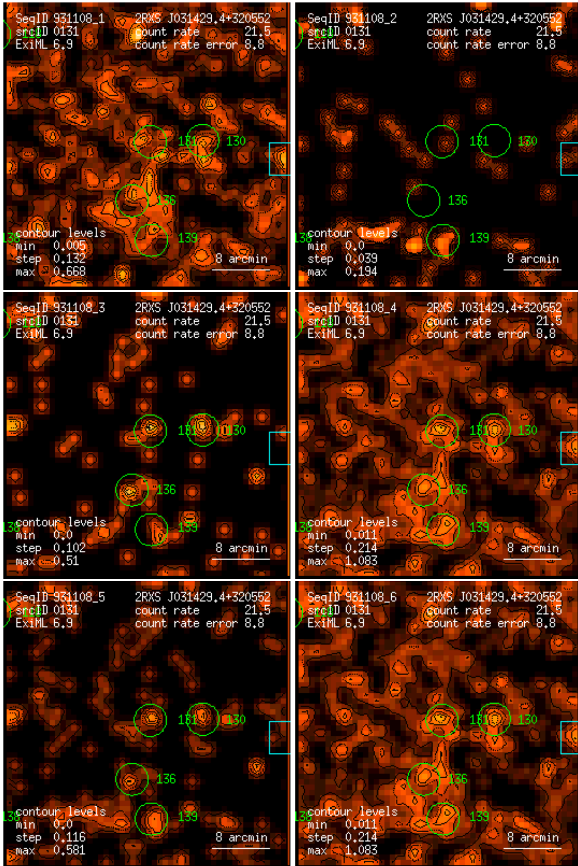
Figure 131: RASS 931108: detection 0131: band rate images, Gaussian filter: (1) PSPC channels 11 – 41, (2) 52 – 90, (3) 91 – 201, (4) 11 – 235, (5) 52 – 201, (6) 11 – 201. Broad band rates in counts/ks. Band rate contour levels in counts/ks/arcmin 2 .
