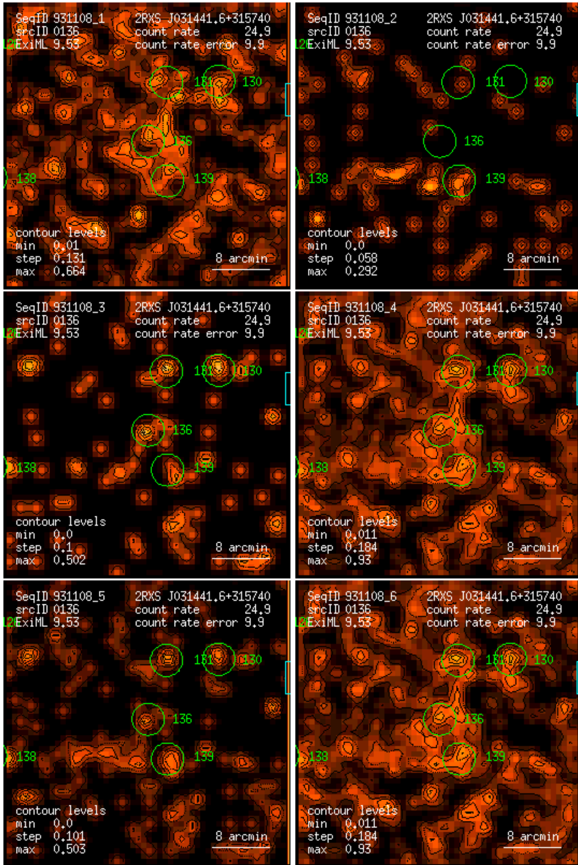
Figure 136: RASS 931108: detection 0136: band rate images, Gaussian filter: (1) PSPC channels 11 – 41, (2) 52 – 90, (3) 91 – 201, (4) 11 – 235, (5) 52 – 201, (6) 11 – 201. Broad band rates in counts/ks. Band rate contour levels in counts/ks/arcmin 2 .
