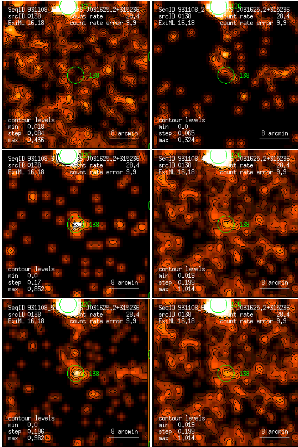
Figure 138: RASS 931108: detection 0138: band rate images, Gaussian filter: (1) PSPC channels 11 – 41, (2) 52 – 90, (3) 91 – 201, (4) 11 – 235, (5) 52 – 201, (6) 11 – 201. Broad band rates in counts/ks. Band rate contour levels in counts/ks/arcmin 2 .
