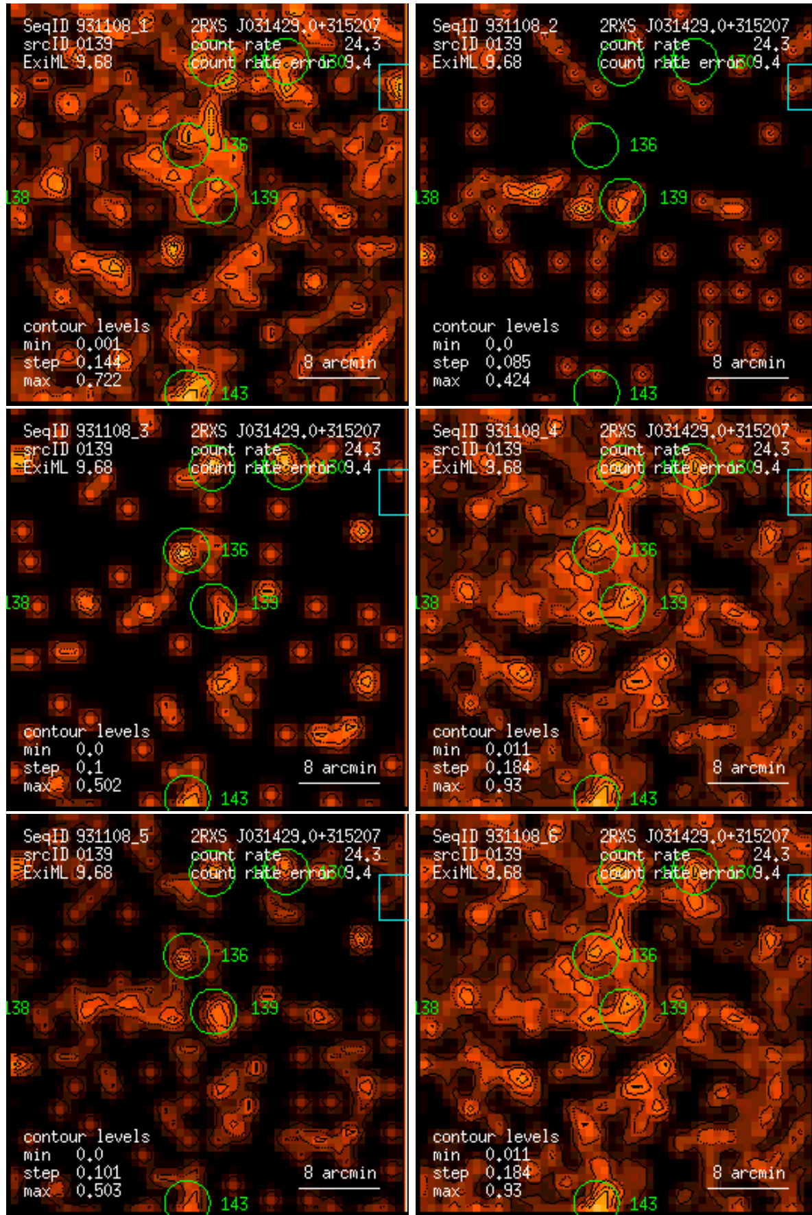
Figure 139: RASS 931108: detection 0139: band rate images, Gaussian filter: (1) PSPC channels 11 – 41, (2) 52 – 90, (3) 91 – 201, (4) 11 – 235, (5) 52 – 201, (6) 11 – 201. Broad band rates in counts/ks. Band rate contour levels in counts/ks/arcmin 2 .
