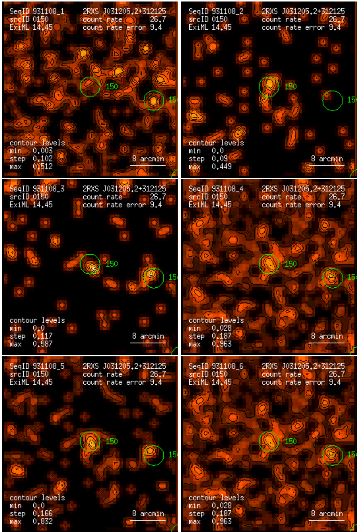
Figure 150: RASS 931108: detection 0150: band rate images, Gaussian filter: (1) PSPC channels 11 – 41, (2) 52 – 90, (3) 91 – 201, (4) 11 – 235, (5) 52 – 201, (6) 11 – 201. Broad band rates in counts/ks. Band rate contour levels in counts/ks/arcmin 2 .
