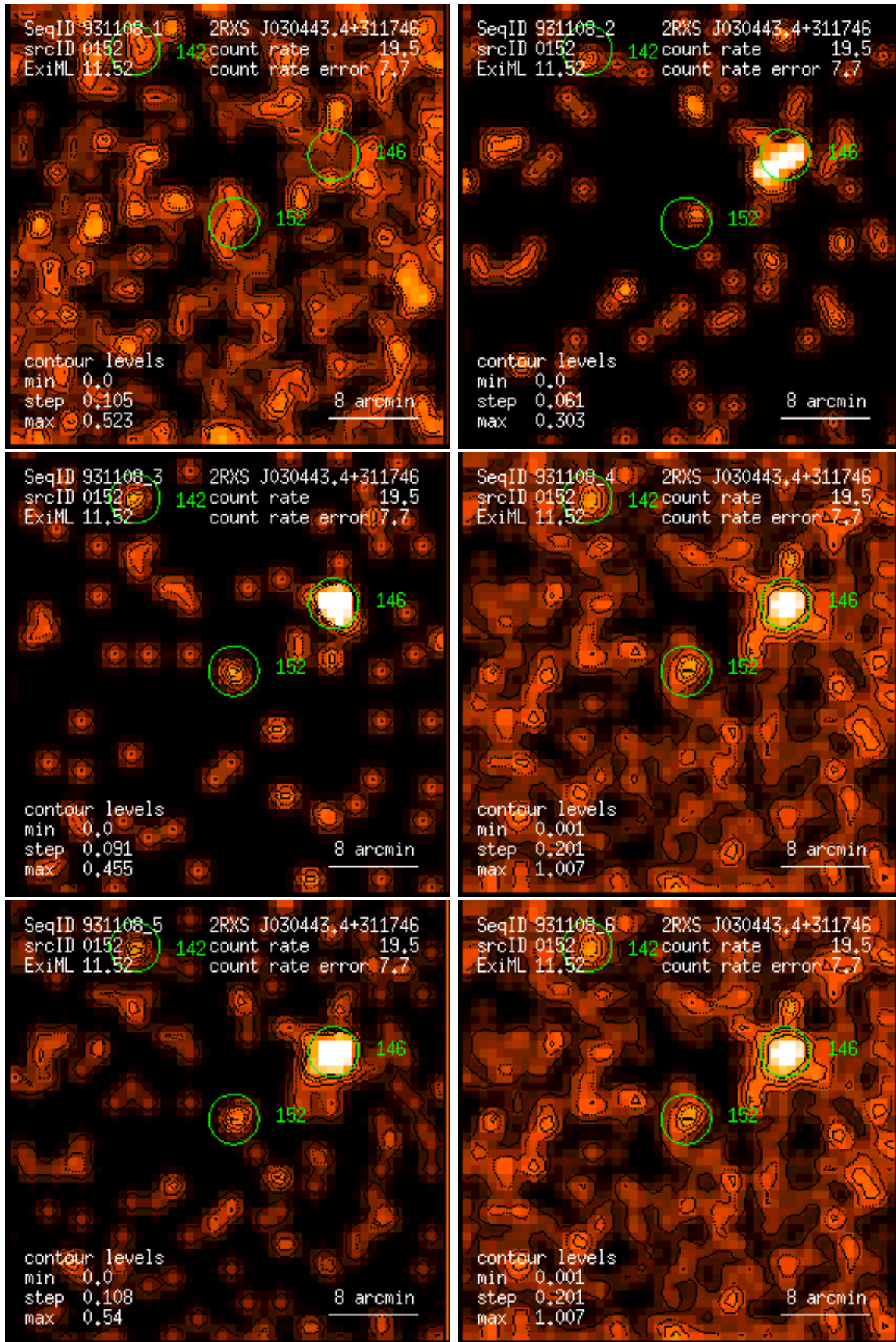
Figure 152: RASS 931108: detection 0152: band rate images, Gaussian filter: (1) PSPC channels 11 – 41, (2) 52 – 90, (3) 91 – 201, (4) 11 – 235, (5) 52 – 201, (6) 11 – 201. Broad band rates in counts/ks. Band rate contour levels in counts/ks/arcmin 2 .
