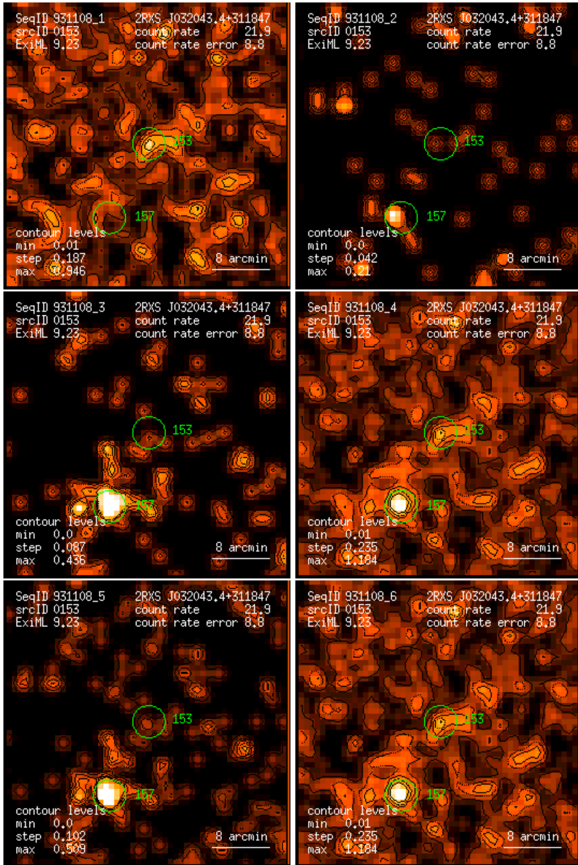
Figure 153: RASS 931108: detection 0153: band rate images, Gaussian filter: (1) PSPC channels 11 – 41, (2) 52 – 90, (3) 91 – 201, (4) 11 – 235, (5) 52 – 201, (6) 11 – 201. Broad band rates in counts/ks. Band rate contour levels in counts/ks/arcmin 2 .
