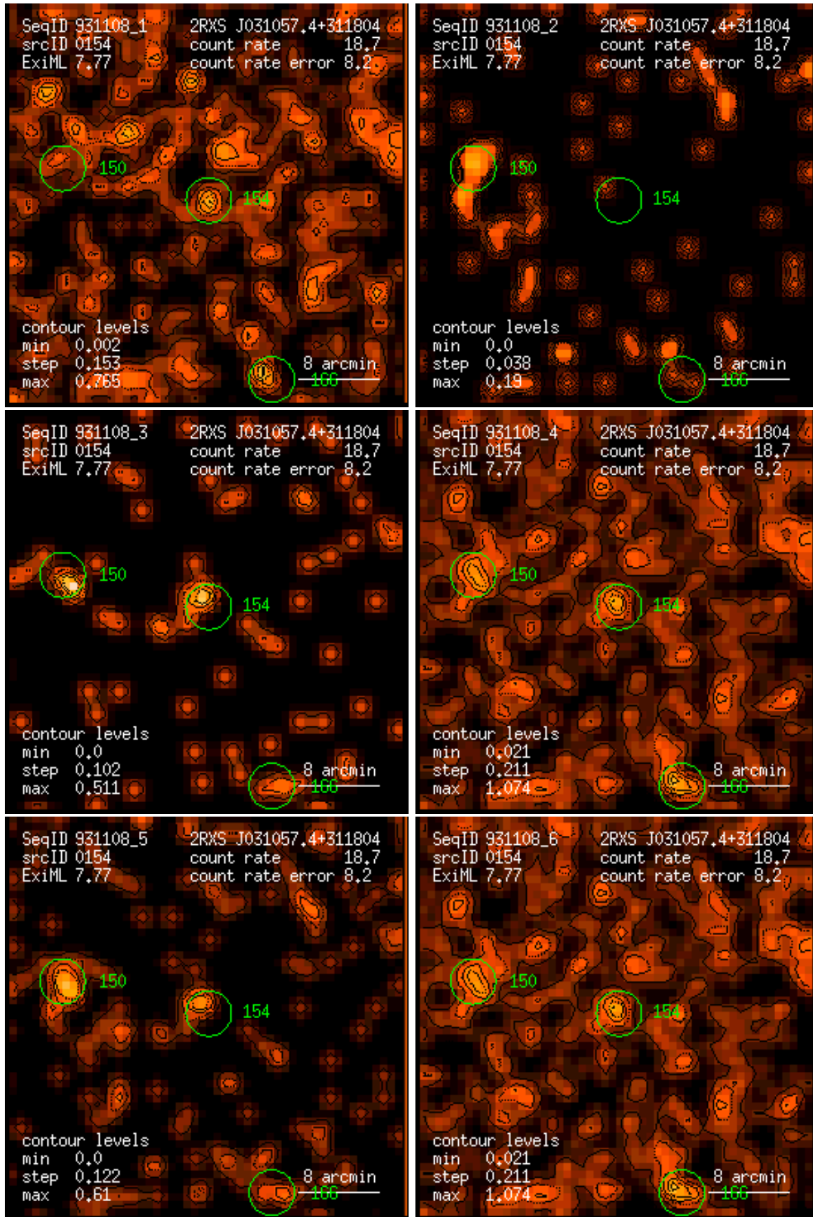
Figure 154: RASS 931108: detection 0154: band rate images, Gaussian filter: (1) PSPC channels 11 – 41, (2) 52 – 90, (3) 91 – 201, (4) 11 – 235, (5) 52 – 201, (6) 11 – 201. Broad band rates in counts/ks. Band rate contour levels in counts/ks/arcmin 2 .
