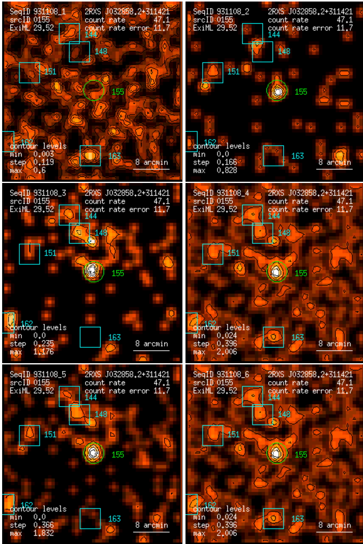
Figure 155: RASS 931108: detection 0155: band rate images, Gaussian filter: (1) PSPC channels 11 – 41, (2) 52 – 90, (3) 91 – 201, (4) 11 – 235, (5) 52 – 201, (6) 11 – 201. Broad band rates in counts/ks. Band rate contour levels in counts/ks/arcmin 2 .
