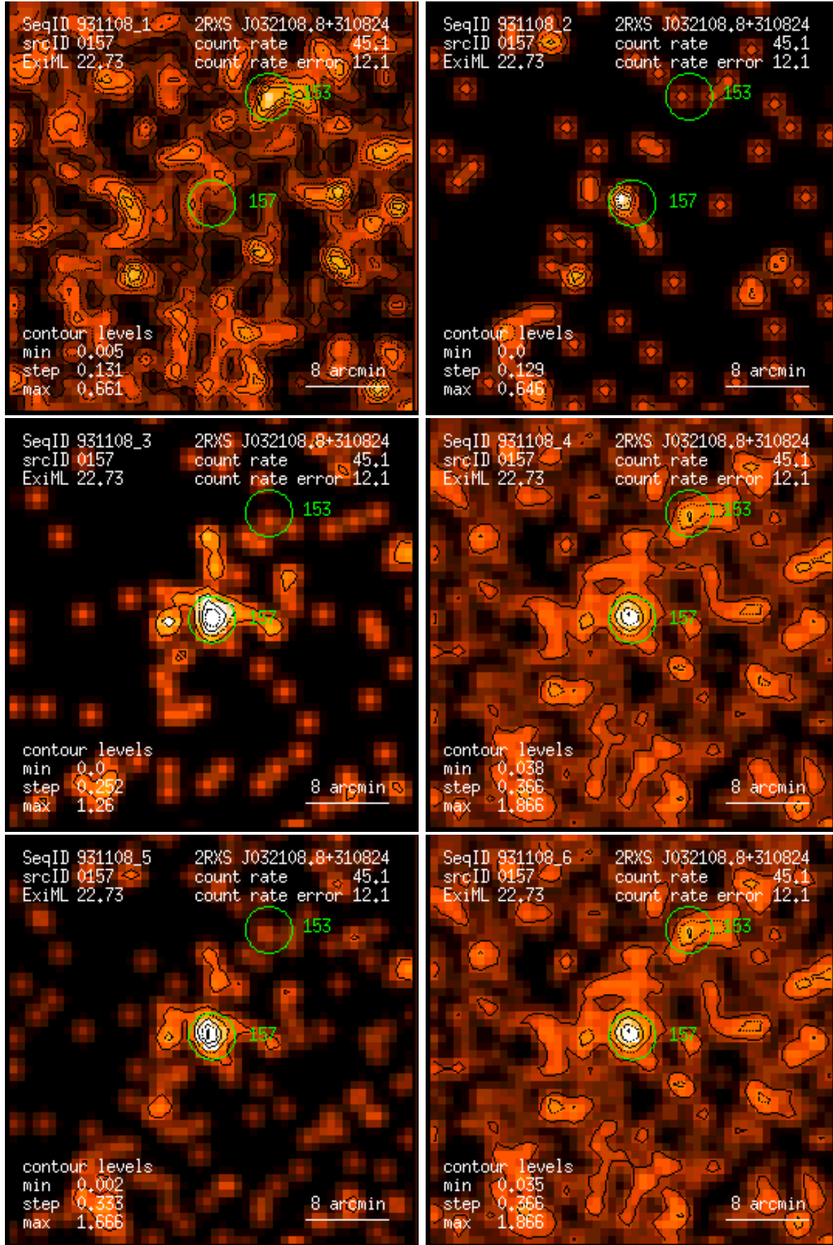
Figure 157: RASS 931108: detection 0157: band rate images, Gaussian filter: (1) PSPC channels 11 – 41, (2) 52 – 90, (3) 91 – 201, (4) 11 – 235, (5) 52 – 201, (6) 11 – 201. Broad band rates in counts/ks. Band rate contour levels in counts/ks/arcmin 2 .
