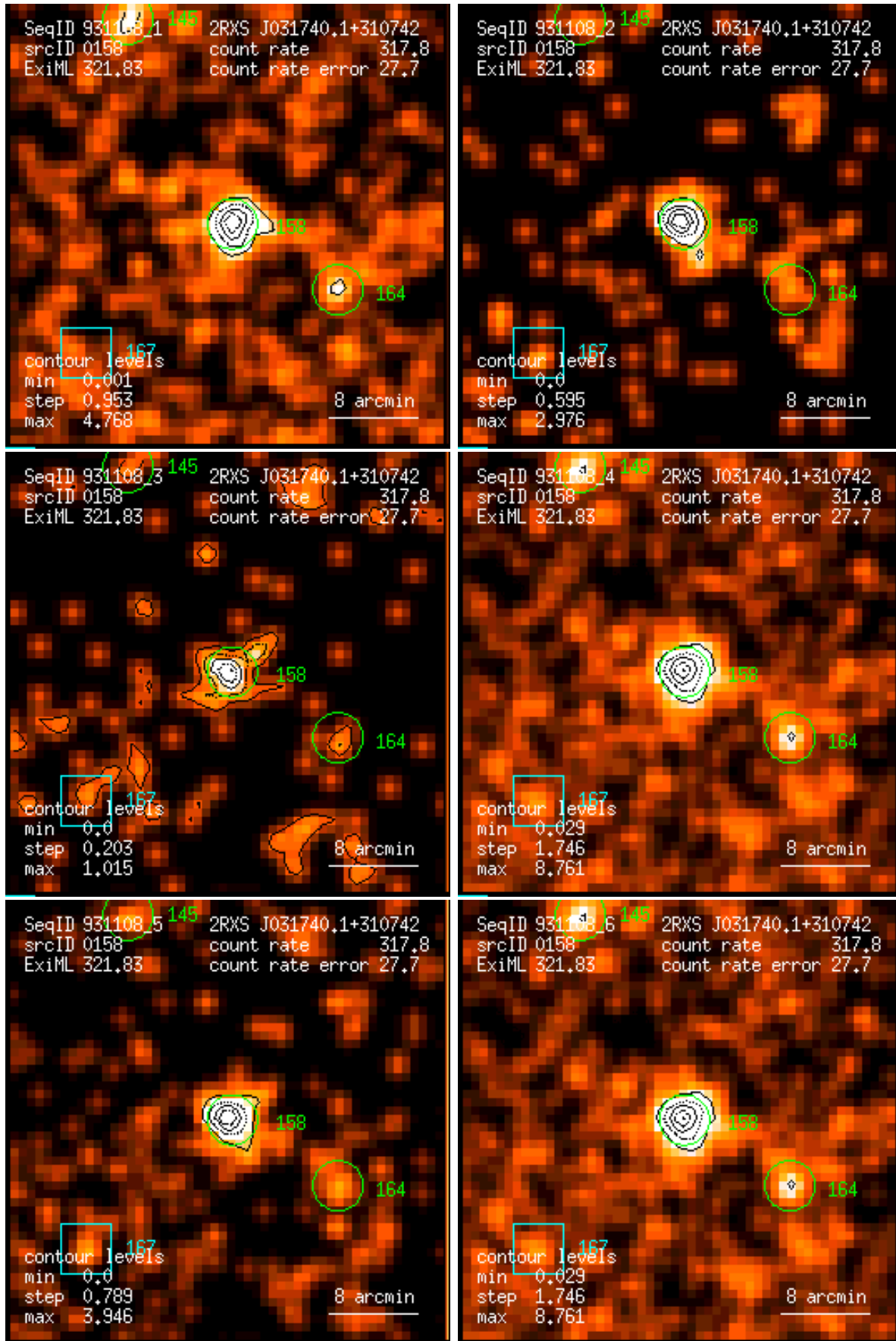
Figure 158: RASS 931108: detection 0158: band rate images, Gaussian filter: (1) PSPC channels 11 – 41, (2) 52 – 90, (3) 91 – 201, (4) 11 – 235, (5) 52 – 201, (6) 11 – 201. Broad band rates in counts/ks. Band rate contour levels in counts/ks/arcmin 2 .
