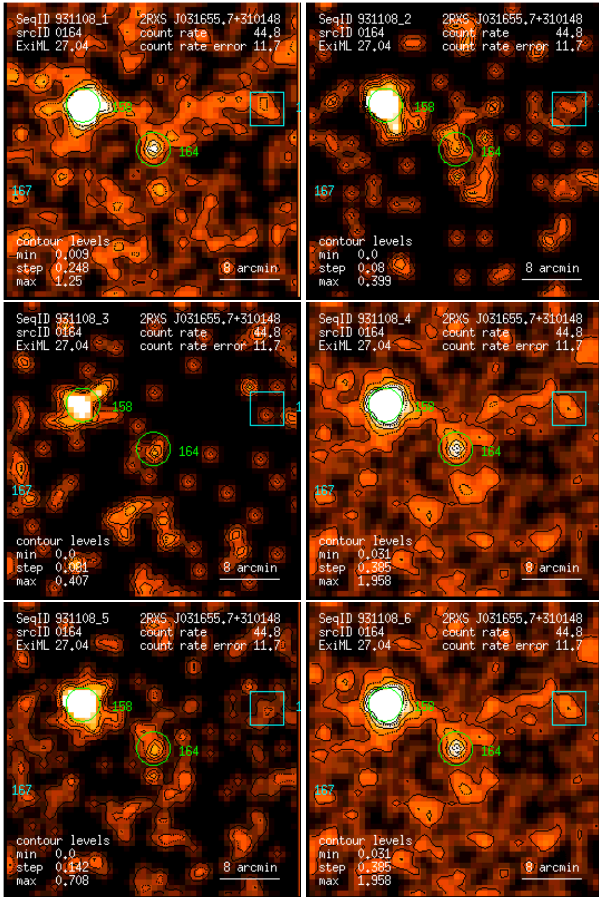
Figure 164: RASS 931108: detection 0164: band rate images, Gaussian filter: (1) PSPC channels 11 – 41, (2) 52 – 90, (3) 91 – 201, (4) 11 – 235, (5) 52 – 201, (6) 11 – 201. Broad band rates in counts/ks. Band rate contour levels in counts/ks/arcmin 2 .
