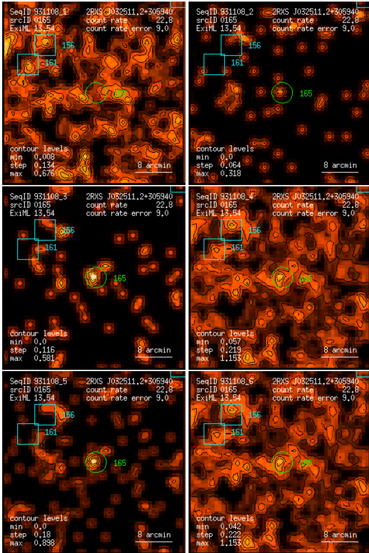
Figure 165: RASS 931108: detection 0165: band rate images, Gaussian filter: (1) PSPC channels 11 – 41, (2) 52 – 90, (3) 91 – 201, (4) 11 – 235, (5) 52 – 201, (6) 11 – 201. Broad band rates in counts/ks. Band rate contour levels in counts/ks/arcmin 2 .
