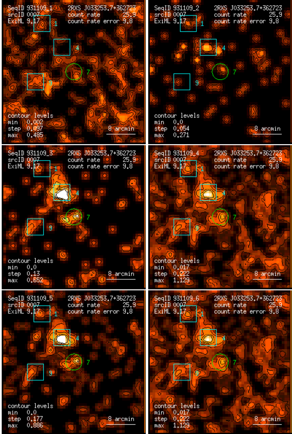
Figure 7: RASS 931109: detection 0007: band rate images, Gaussian filter: (1) PSPC channels 11 – 41, (2) 52 – 90, (3) 91 – 201, (4) 11 – 235, (5) 52 – 201, (6) 11 – 201. Broad band rates in counts/ks. Band rate contour levels in counts/ks/arcmin 2 .
