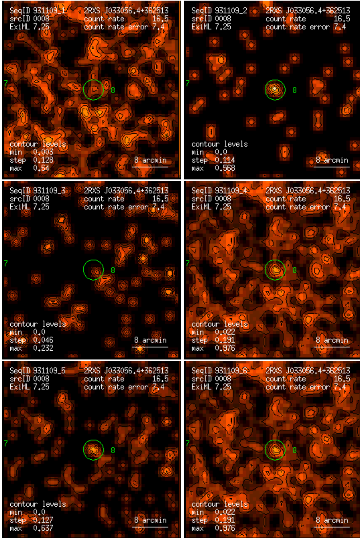
Figure 8: RASS 931109: detection 0008: band rate images, Gaussian filter: (1) PSPC channels 11 – 41, (2) 52 – 90, (3) 91 – 201, (4) 11 – 235, (5) 52 – 201, (6) 11 – 201. Broad band rates in counts/ks. Band rate contour levels in counts/ks/arcmin 2 .
