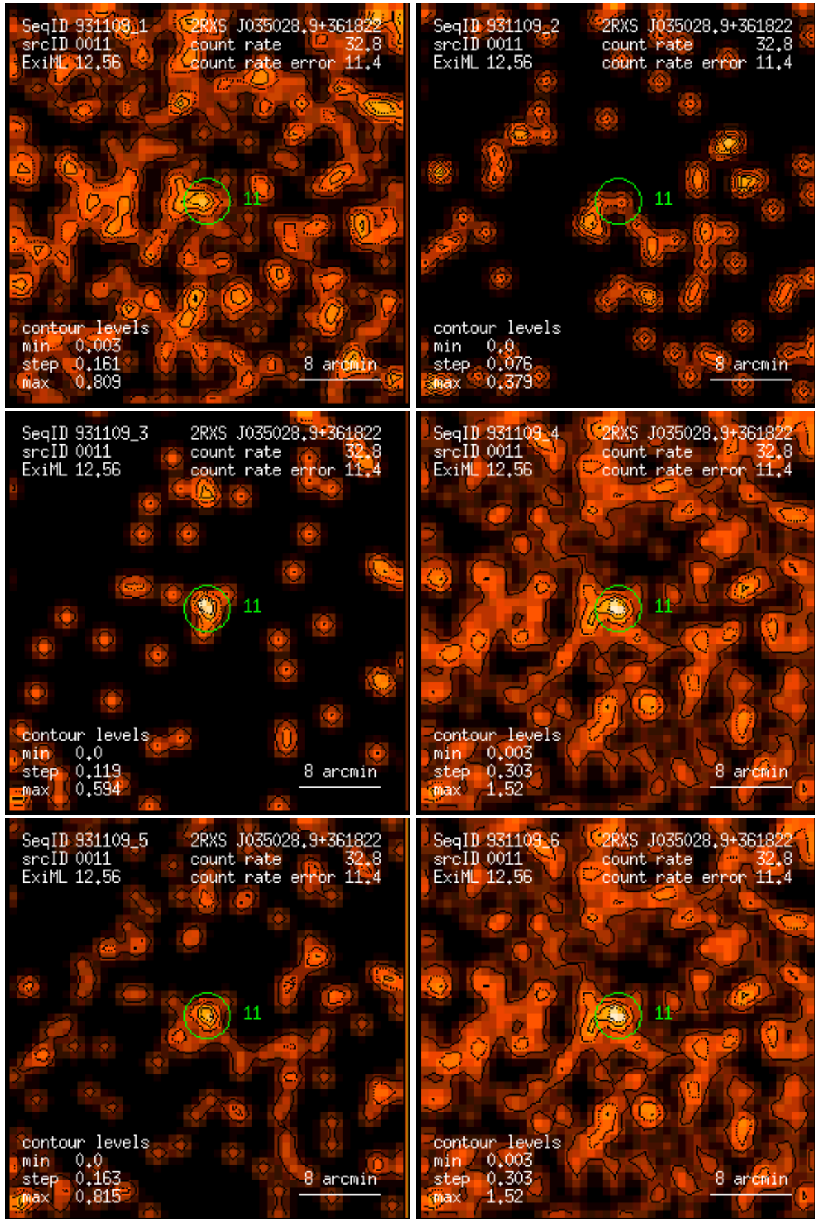
Figure 11: RASS 931109: detection 0011: band rate images, Gaussian filter: (1) PSPC channels 11 – 41, (2) 52 – 90, (3) 91 – 201, (4) 11 – 235, (5) 52 – 201, (6) 11 – 201. Broad band rates in counts/ks. Band rate contour levels in counts/ks/arcmin 2 .
