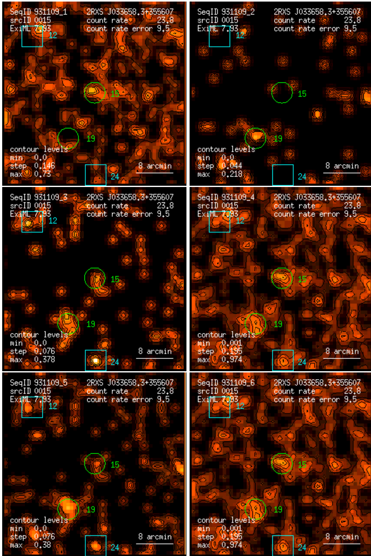
Figure 15: RASS 931109: detection 0015: band rate images, Gaussian filter: (1) PSPC channels 11 – 41, (2) 52 – 90, (3) 91 – 201, (4) 11 – 235, (5) 52 – 201, (6) 11 – 201. Broad band rates in counts/ks. Band rate contour levels in counts/ks/arcmin 2 .
