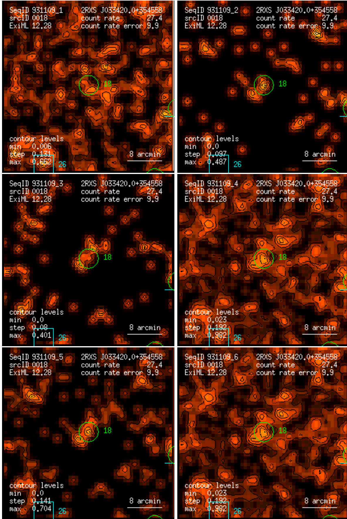
Figure 18: RASS 931109: detection 0018: band rate images, Gaussian filter: (1) PSPC channels 11 – 41, (2) 52 – 90, (3) 91 – 201, (4) 11 – 235, (5) 52 – 201, (6) 11 – 201. Broad band rates in counts/ks. Band rate contour levels in counts/ks/arcmin 2 .
