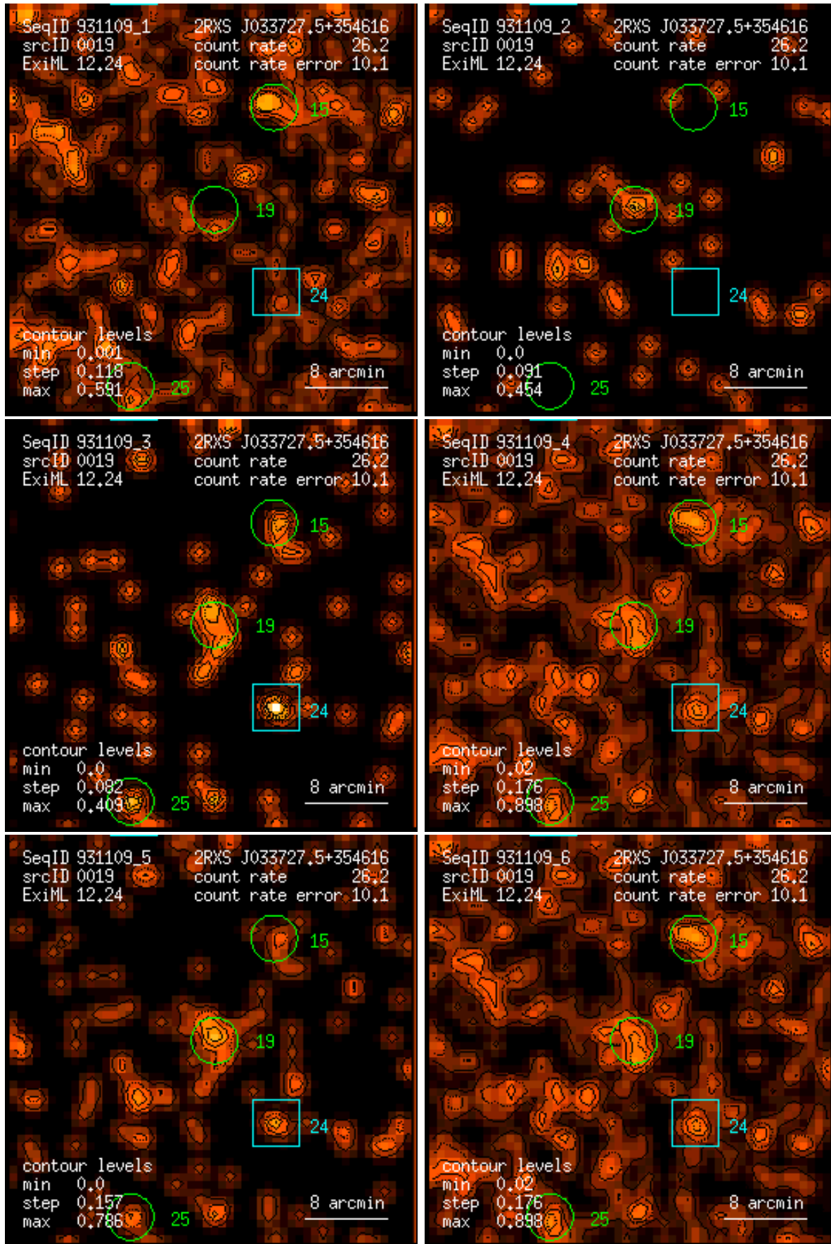
Figure 19: RASS 931109: detection 0019: band rate images, Gaussian filter: (1) PSPC channels 11 – 41, (2) 52 – 90, (3) 91 – 201, (4) 11 – 235, (5) 52 – 201, (6) 11 – 201. Broad band rates in counts/ks. Band rate contour levels in counts/ks/arcmin 2 .
