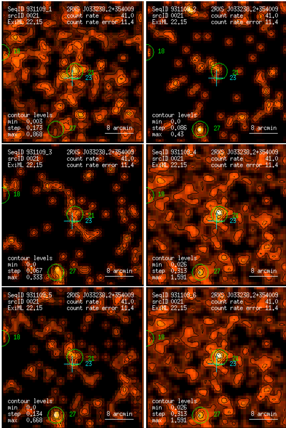
Figure 21: RASS 931109: detection 0021: band rate images, Gaussian filter: (1) PSPC channels 11 – 41, (2) 52 – 90, (3) 91 – 201, (4) 11 – 235, (5) 52 – 201, (6) 11 – 201. Broad band rates in counts/ks. Band rate contour levels in counts/ks/arcmin 2 .
