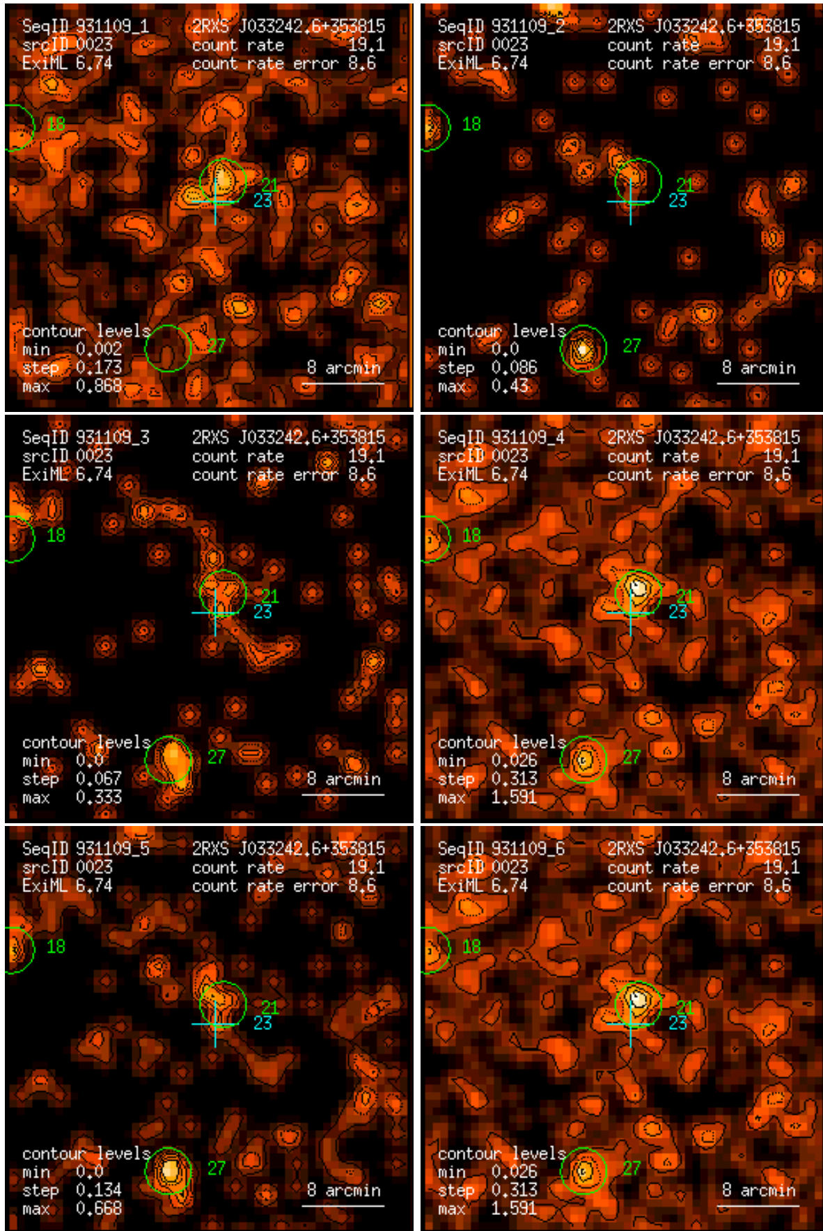
Figure 23: RASS 931109: detection 0023: band rate images, Gaussian filter: (1) PSPC channels 11 – 41, (2) 52 – 90, (3) 91 – 201, (4) 11 – 235, (5) 52 – 201, (6) 11 – 201. Broad band rates in counts/ks. Band rate contour levels in counts/ks/arcmin 2 .
