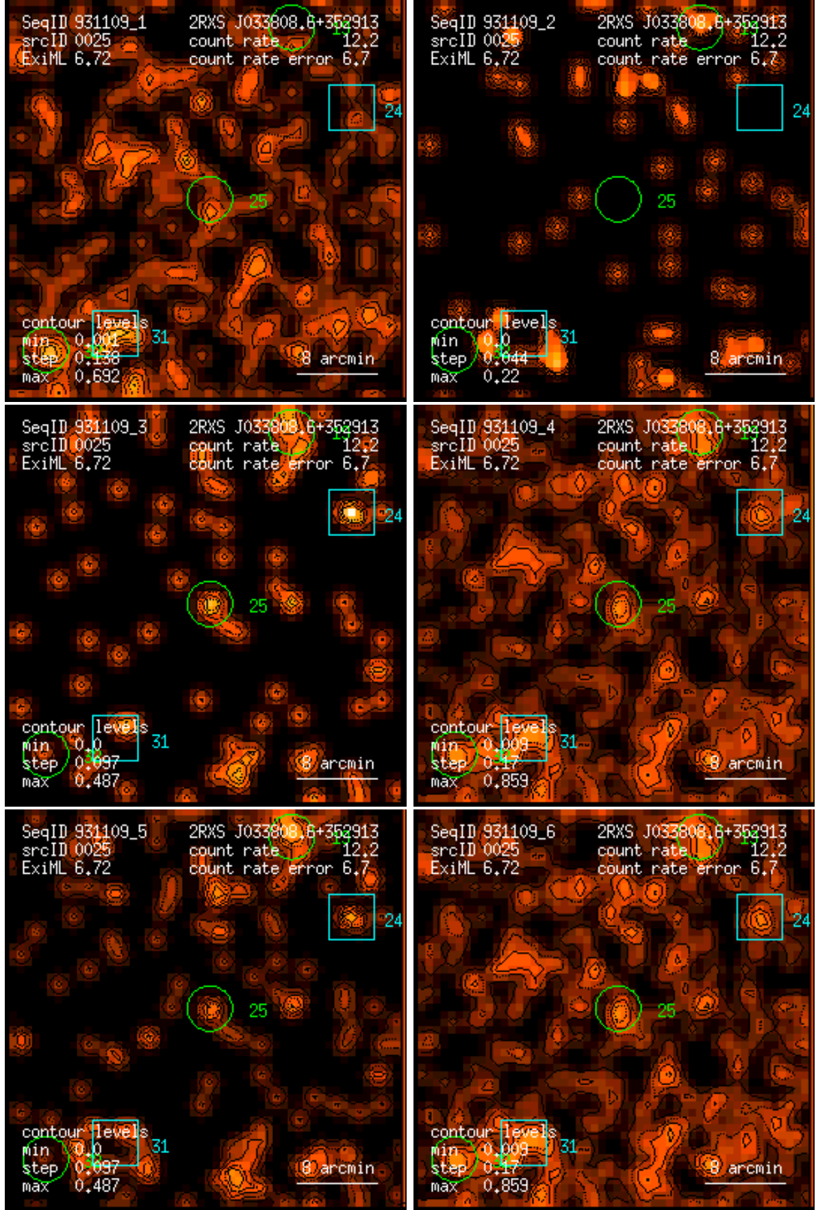
Figure 25: RASS 931109: detection 0025: band rate images, Gaussian filter: (1) PSPC channels 11 – 41, (2) 52 – 90, (3) 91 – 201, (4) 11 – 235, (5) 52 – 201, (6) 11 – 201. Broad band rates in counts/ks. Band rate contour levels in counts/ks/arcmin 2 .
