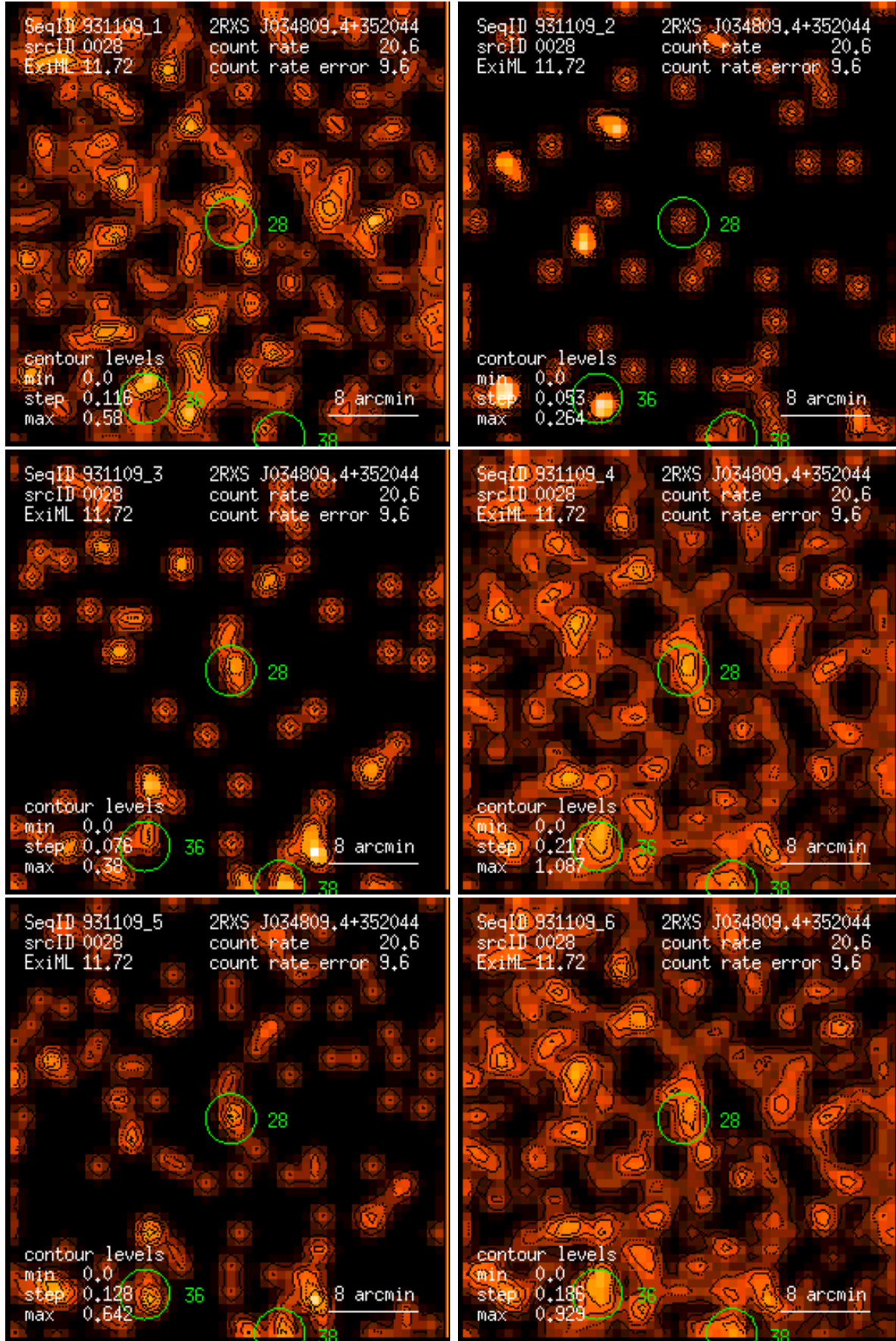
Figure 28: RASS 931109: detection 0028: band rate images, Gaussian filter: (1) PSPC channels 11 – 41, (2) 52 – 90, (3) 91 – 201, (4) 11 – 235, (5) 52 – 201, (6) 11 – 201. Broad band rates in counts/ks. Band rate contour levels in counts/ks/arcmin 2 .
