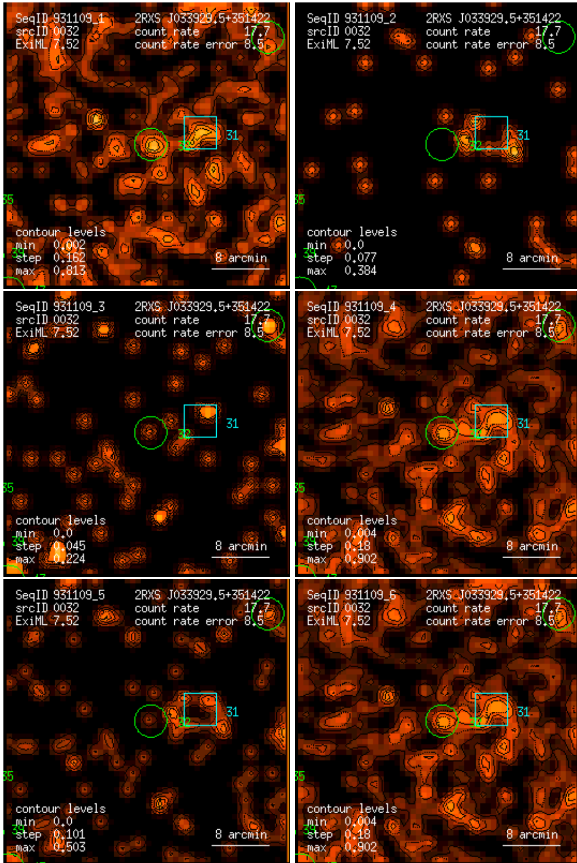
Figure 32: RASS 931109: detection 0032: band rate images, Gaussian filter: (1) PSPC channels 11 – 41, (2) 52 – 90, (3) 91 – 201, (4) 11 – 235, (5) 52 – 201, (6) 11 – 201. Broad band rates in counts/ks. Band rate contour levels in counts/ks/arcmin 2 .
