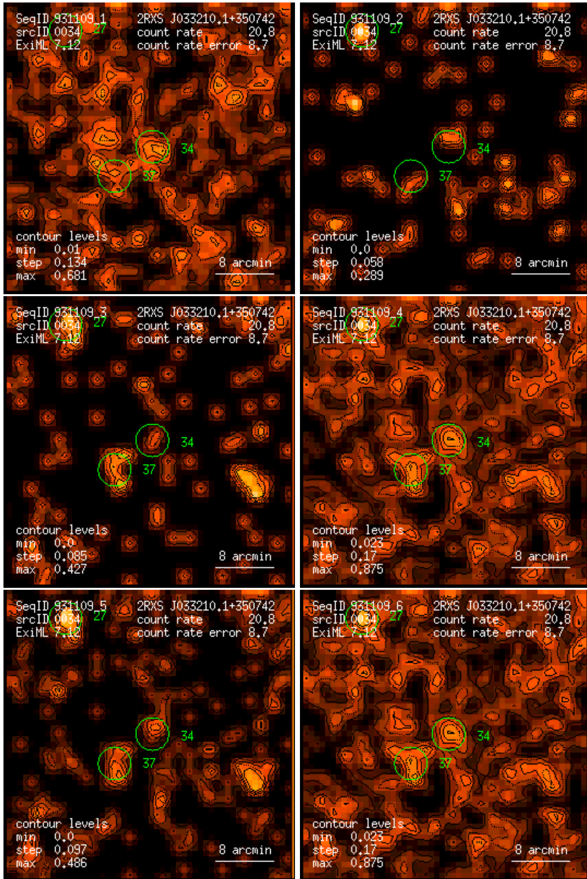
Figure 34: RASS 931109: detection 0034: band rate images, Gaussian filter: (1) PSPC channels 11 – 41, (2) 52 – 90, (3) 91 – 201, (4) 11 – 235, (5) 52 – 201, (6) 11 – 201. Broad band rates in counts/ks. Band rate contour levels in counts/ks/arcmin 2 .
