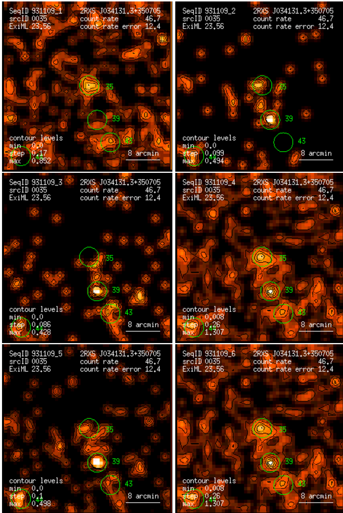
Figure 35: RASS 931109: detection 0035: band rate images, Gaussian filter: (1) PSPC channels 11 – 41, (2) 52 – 90, (3) 91 – 201, (4) 11 – 235, (5) 52 – 201, (6) 11 – 201. Broad band rates in counts/ks. Band rate contour levels in counts/ks/arcmin 2 .
