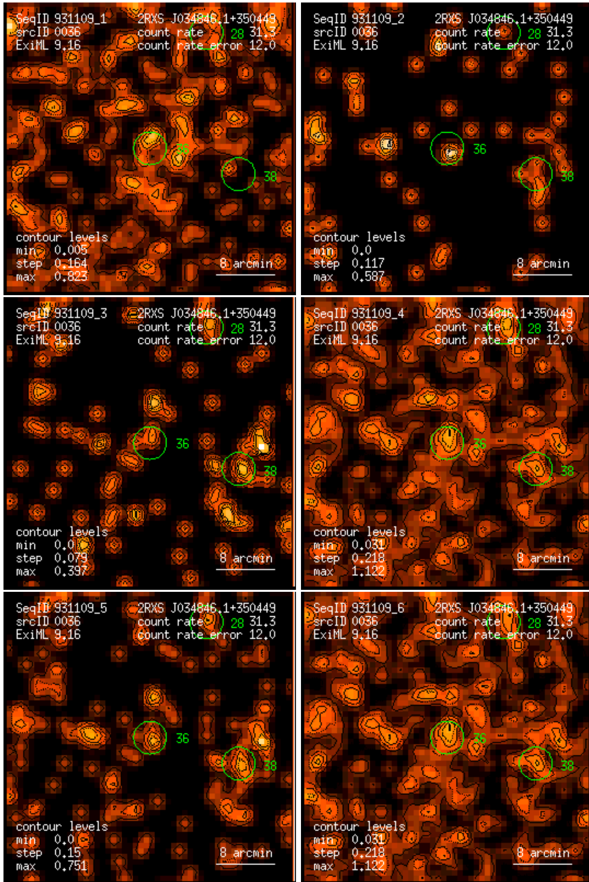
Figure 36: RASS 931109: detection 0036: band rate images, Gaussian filter: (1) PSPC channels 11 – 41, (2) 52 – 90, (3) 91 – 201, (4) 11 – 235, (5) 52 – 201, (6) 11 – 201. Broad band rates in counts/ks. Band rate contour levels in counts/ks/arcmin 2 .
