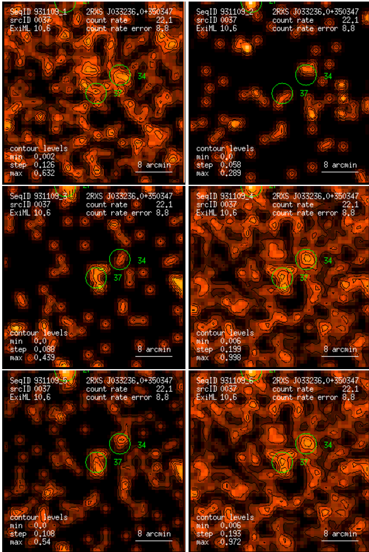
Figure 37: RASS 931109: detection 0037: band rate images, Gaussian filter: (1) PSPC channels 11 – 41, (2) 52 – 90, (3) 91 – 201, (4) 11 – 235, (5) 52 – 201, (6) 11 – 201. Broad band rates in counts/ks. Band rate contour levels in counts/ks/arcmin 2 .
