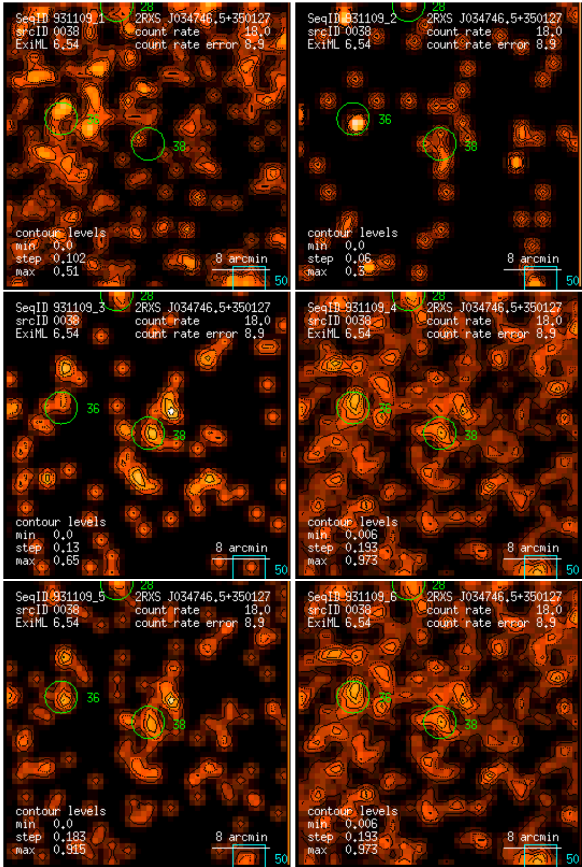
Figure 38: RASS 931109: detection 0038: band rate images, Gaussian filter: (1) PSPC channels 11 – 41, (2) 52 – 90, (3) 91 – 201, (4) 11 – 235, (5) 52 – 201, (6) 11 – 201. Broad band rates in counts/ks. Band rate contour levels in counts/ks/arcmin 2 .
