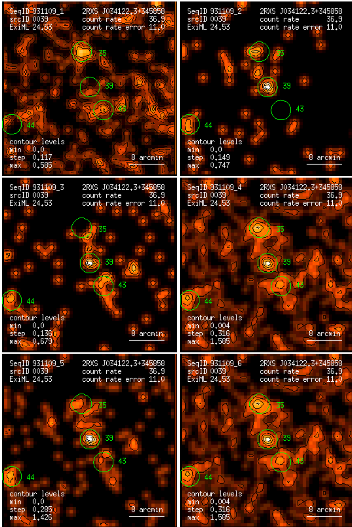
Figure 39: RASS 931109: detection 0039: band rate images, Gaussian filter: (1) PSPC channels 11 – 41, (2) 52 – 90, (3) 91 – 201, (4) 11 – 235, (5) 52 – 201, (6) 11 – 201. Broad band rates in counts/ks. Band rate contour levels in counts/ks/arcmin 2 .
