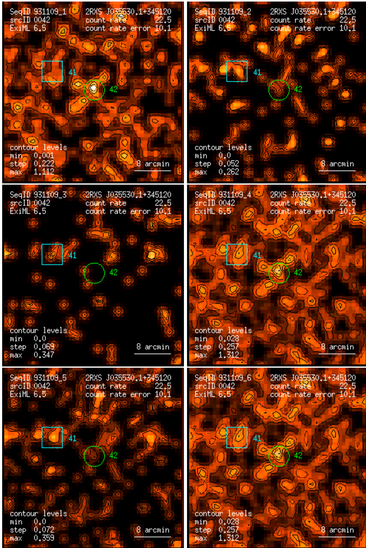
Figure 42: RASS 931109: detection 0042: band rate images, Gaussian filter: (1) PSPC channels 11 – 41, (2) 52 – 90, (3) 91 – 201, (4) 11 – 235, (5) 52 – 201, (6) 11 – 201. Broad band rates in counts/ks. Band rate contour levels in counts/ks/arcmin 2 .
