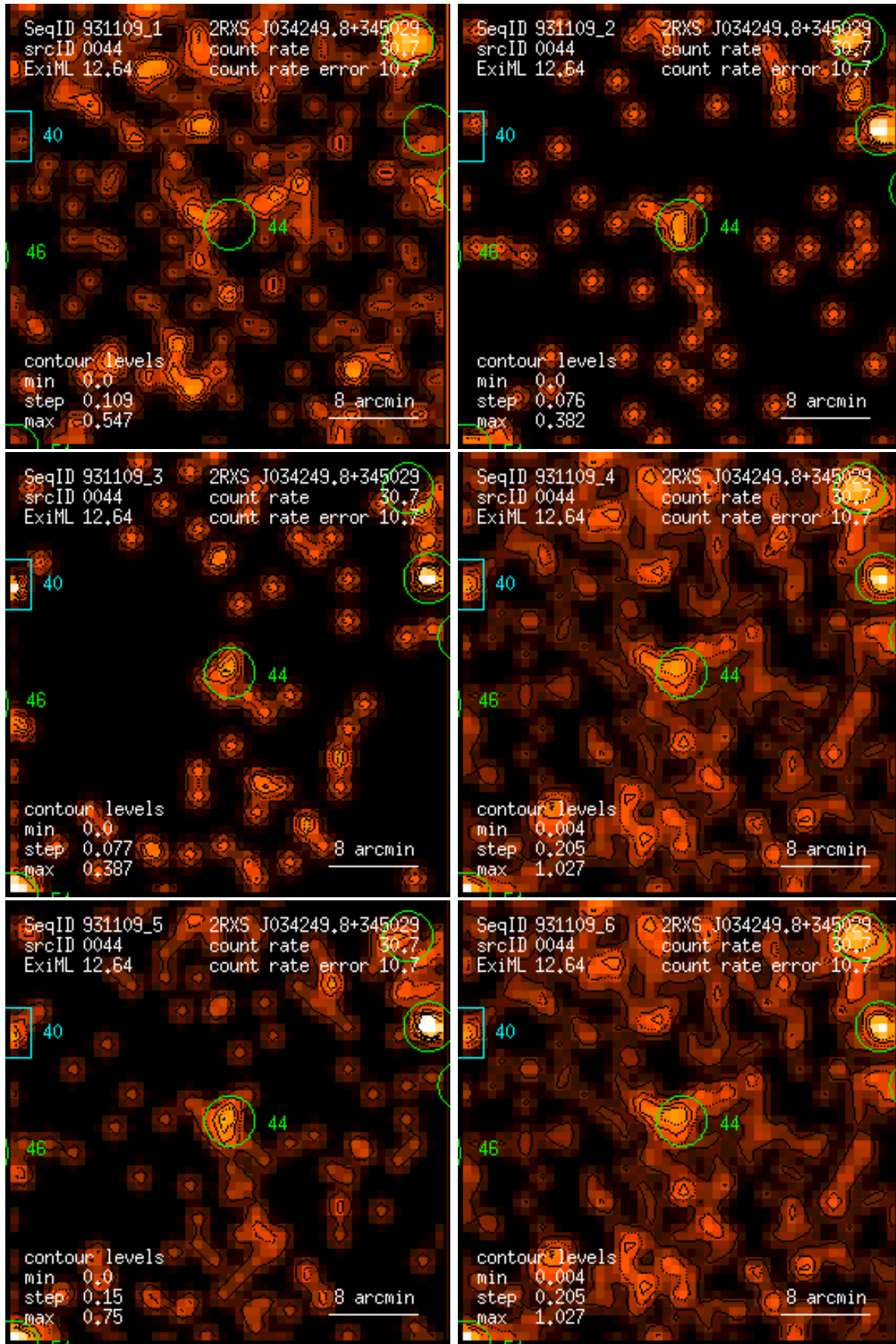
Figure 44: RASS 931109: detection 0044: band rate images, Gaussian filter: (1) PSPC channels 11 – 41, (2) 52 – 90, (3) 91 – 201, (4) 11 – 235, (5) 52 – 201, (6) 11 – 201. Broad band rates in counts/ks. Band rate contour levels in counts/ks/arcmin 2 .
