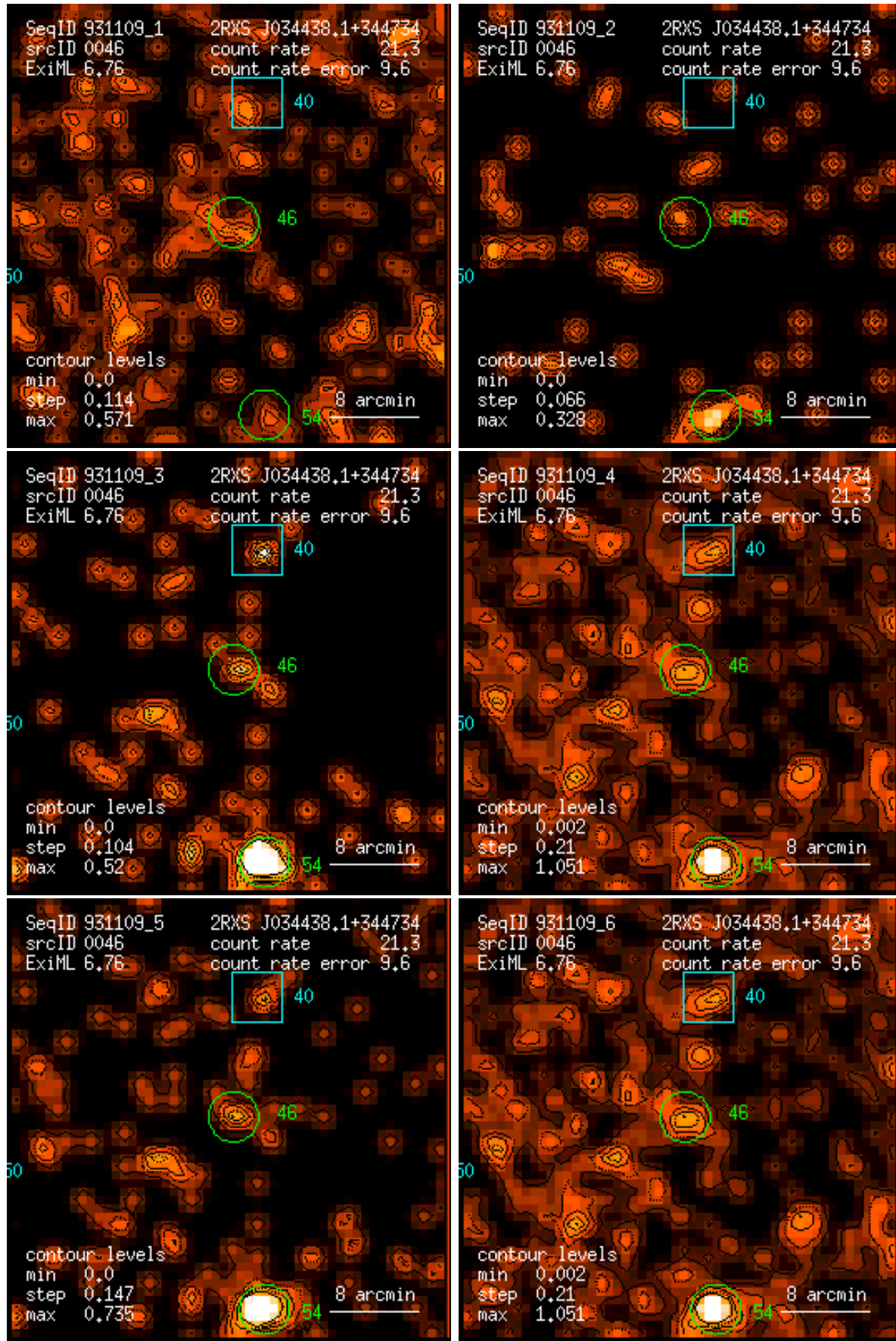
Figure 46: RASS 931109: detection 0046: band rate images, Gaussian filter: (1) PSPC channels 11 – 41, (2) 52 – 90, (3) 91 – 201, (4) 11 – 235, (5) 52 – 201, (6) 11 – 201. Broad band rates in counts/ks. Band rate contour levels in counts/ks/arcmin 2 .
