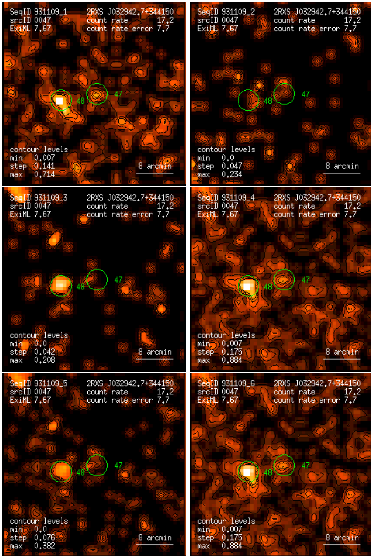
Figure 47: RASS 931109: detection 0047: band rate images, Gaussian filter: (1) PSPC channels 11 – 41, (2) 52 – 90, (3) 91 – 201, (4) 11 – 235, (5) 52 – 201, (6) 11 – 201. Broad band rates in counts/ks. Band rate contour levels in counts/ks/arcmin 2 .
