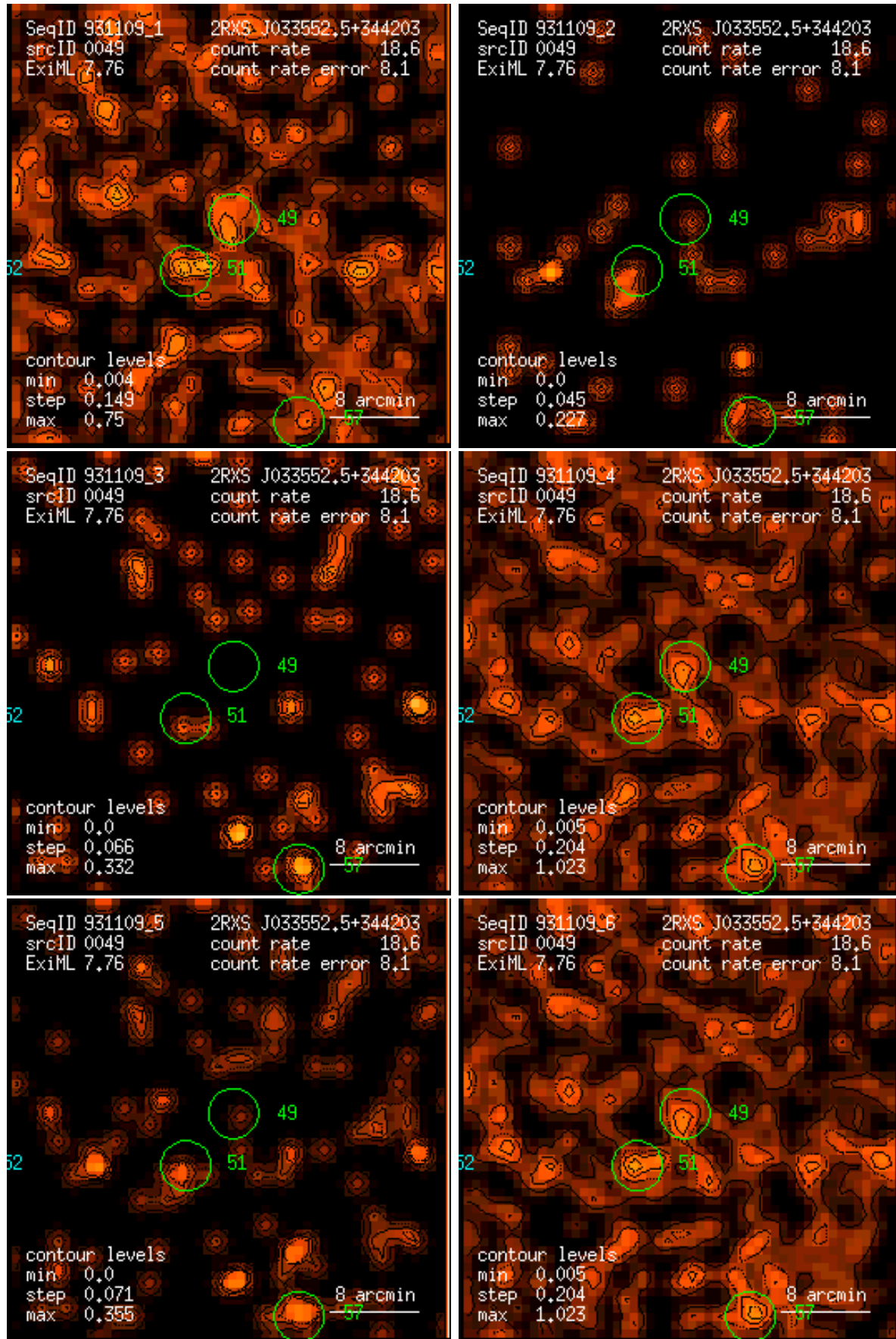
Figure 49: RASS 931109: detection 0049: band rate images, Gaussian filter: (1) PSPC channels 11 – 41, (2) 52 – 90, (3) 91 – 201, (4) 11 – 235, (5) 52 – 201, (6) 11 – 201. Broad band rates in counts/ks. Band rate contour levels in counts/ks/arcmin 2 .
