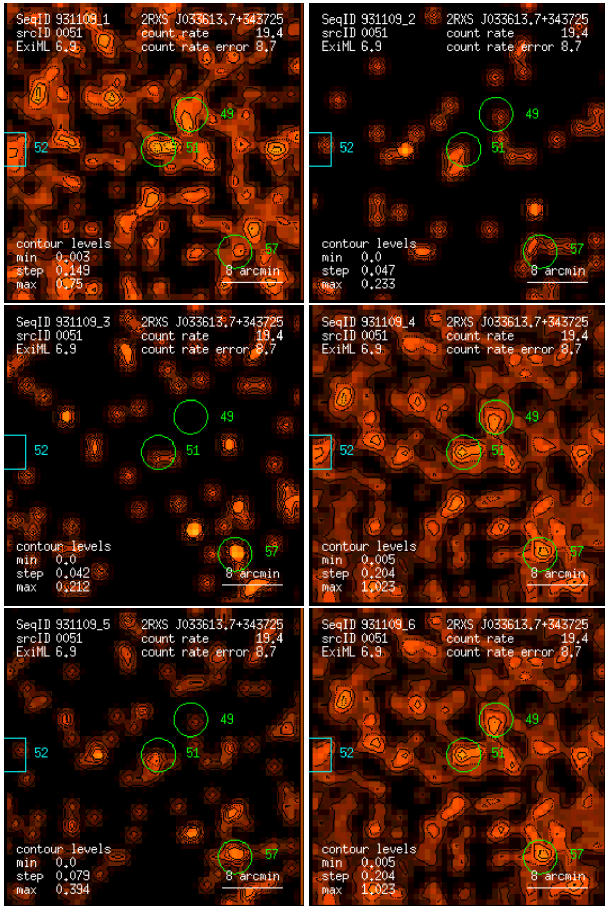
Figure 51: RASS 931109: detection 0051: band rate images, Gaussian filter: (1) PSPC channels 11 – 41, (2) 52 – 90, (3) 91 – 201, (4) 11 – 235, (5) 52 – 201, (6) 11 – 201. Broad band rates in counts/ks. Band rate contour levels in counts/ks/arcmin 2 .
